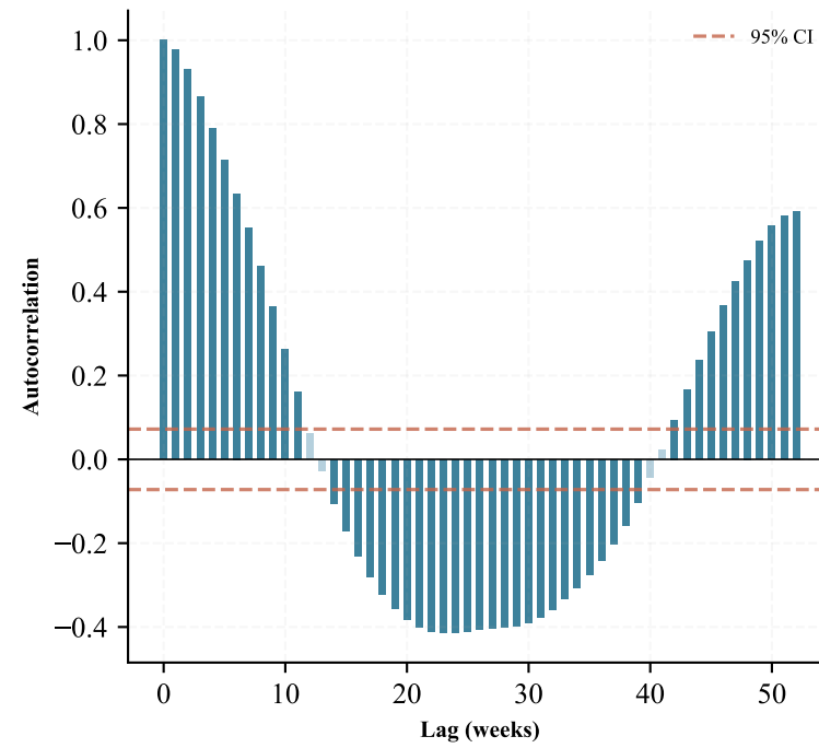
ACF (Lice Outbreak 1m)
