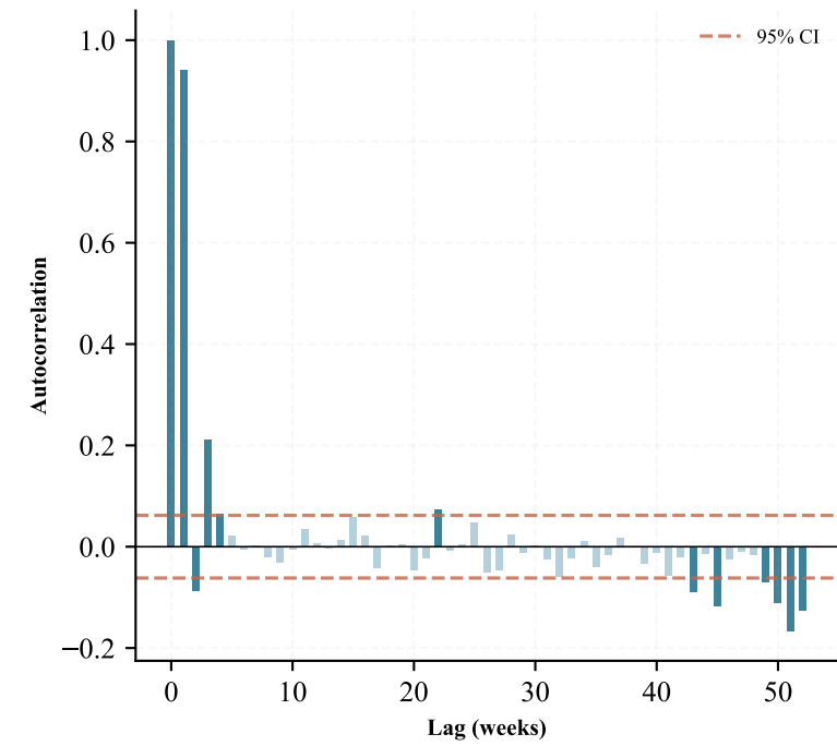
PACF ( \Delta Salmon (NOK/KG) 12m)
