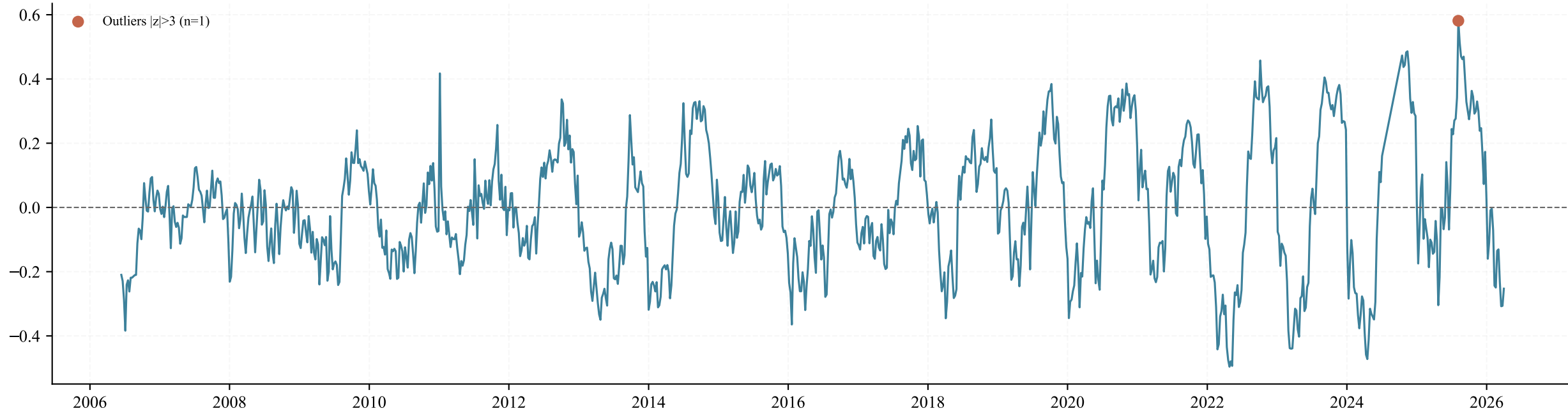
Time Series
