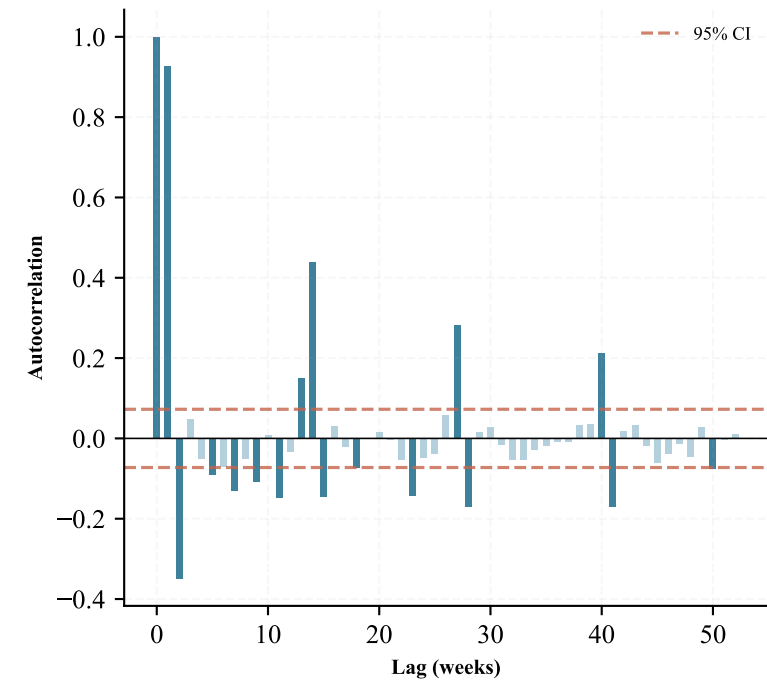
PACF ( \Delta Broiler Price (EU) 3m)
