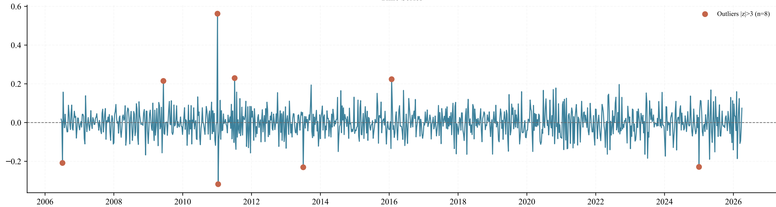
Time Series
