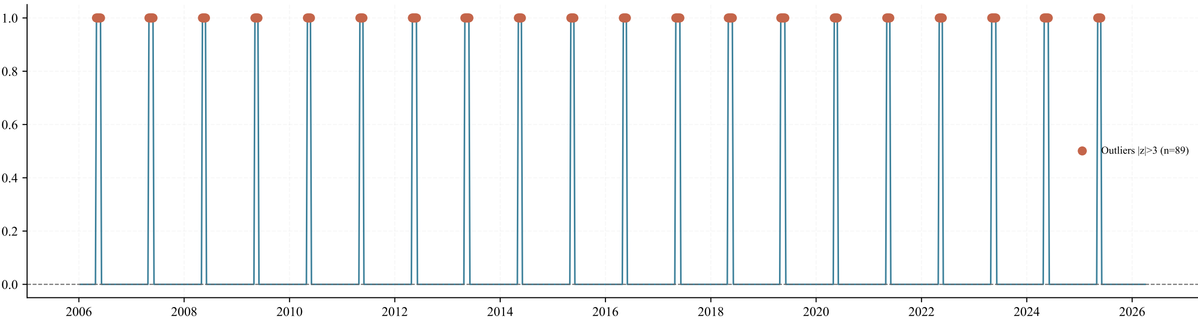
Time Series
