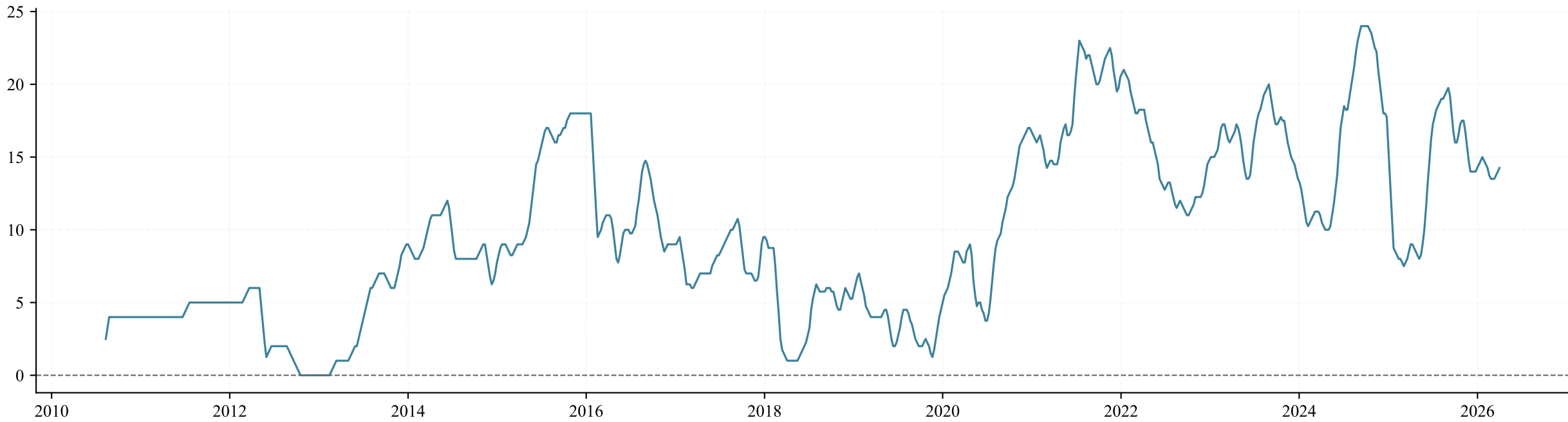
Time Series
