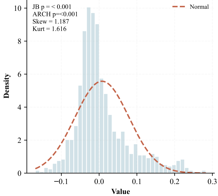
Distribution
