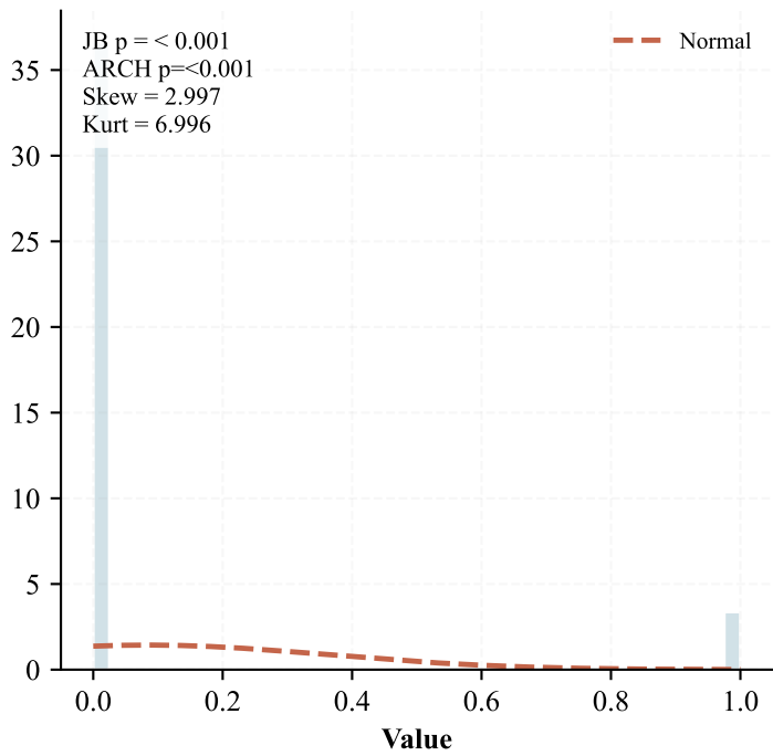
Distribution
