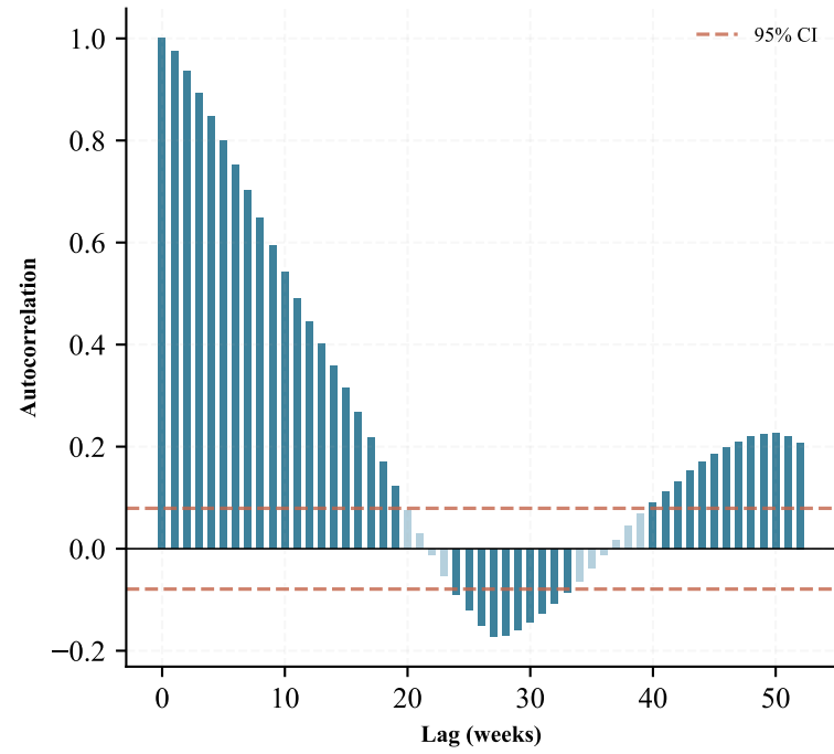
ACF ( \Delta Pig Price (EU) 6m)
