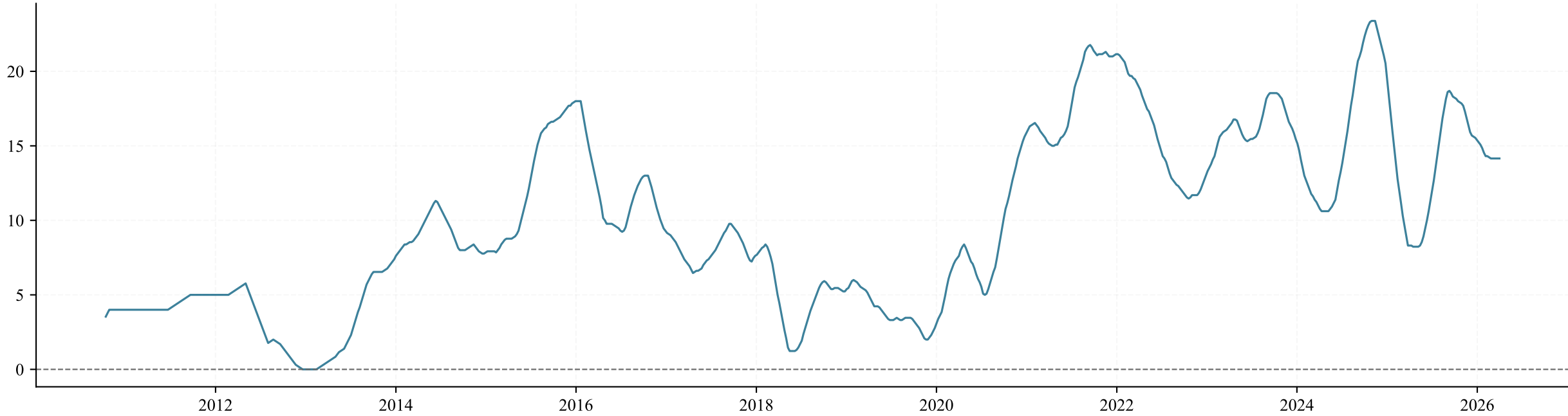
Time Series
