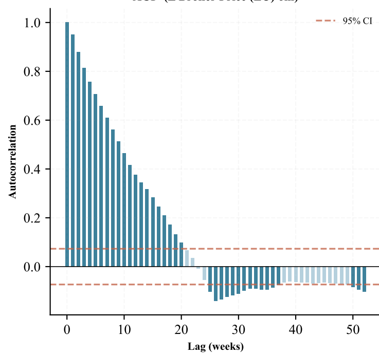
ACF ( \Delta Broiler Price (EU) 6m)
