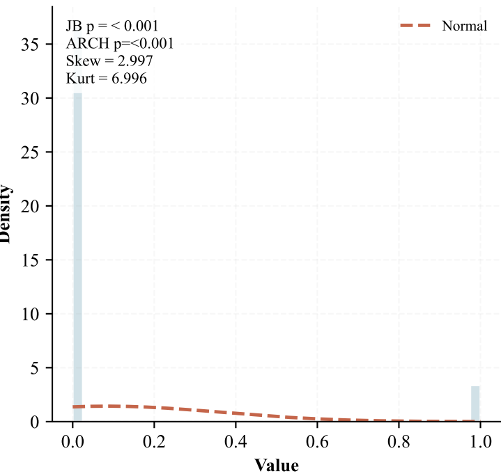
Distribution
