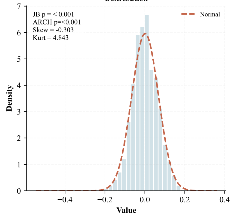
Distribution
