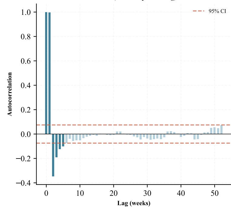
PACF (Sea Temp 12m Avg)
