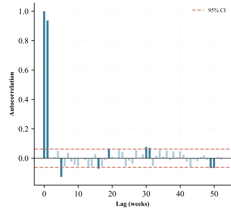
PACF (FWD Slope)
