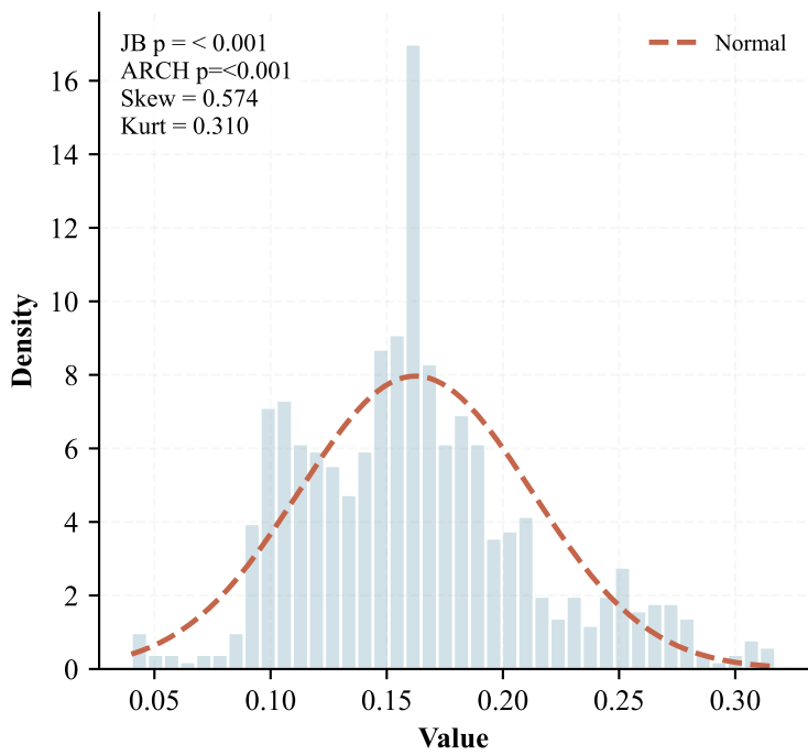
Distribution
