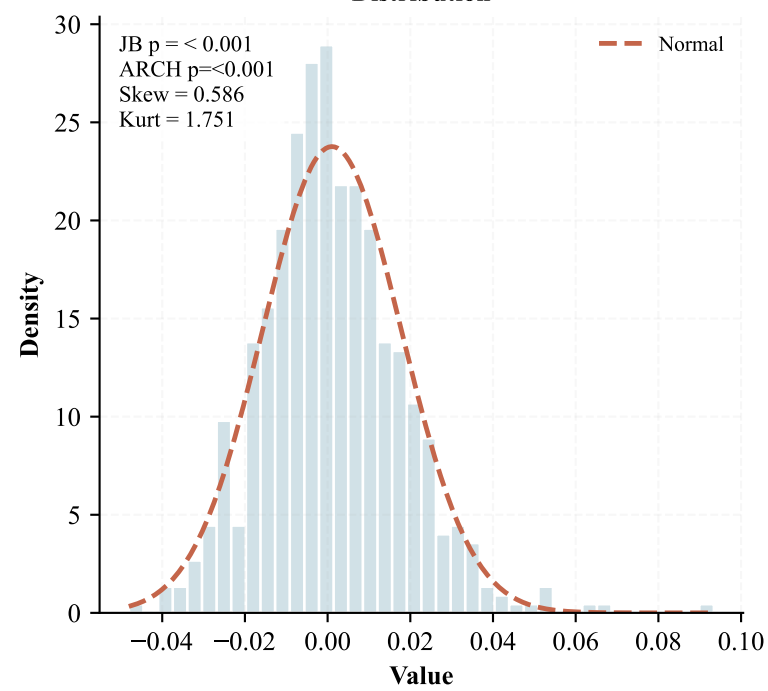
Distribution
