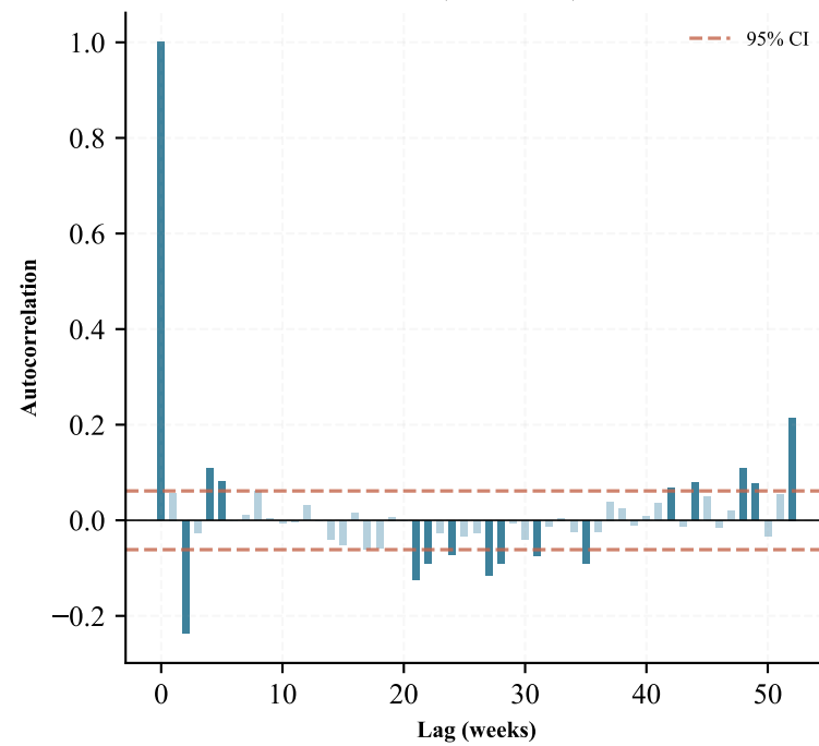
ACF ( \Delta FWD 6m)
