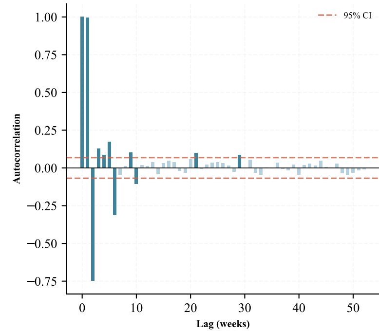
PACF (ISA Outbreak 1m)
