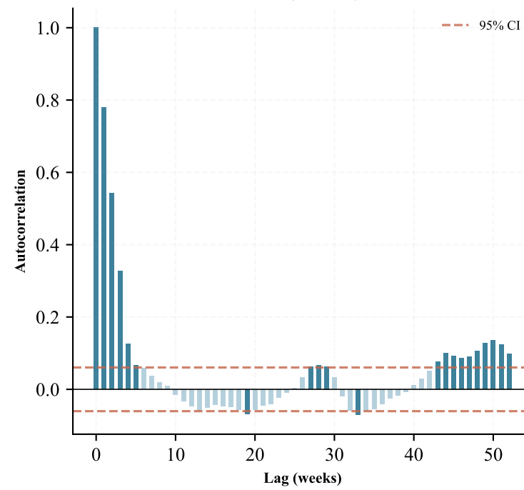
ACF (RVol 4w)
