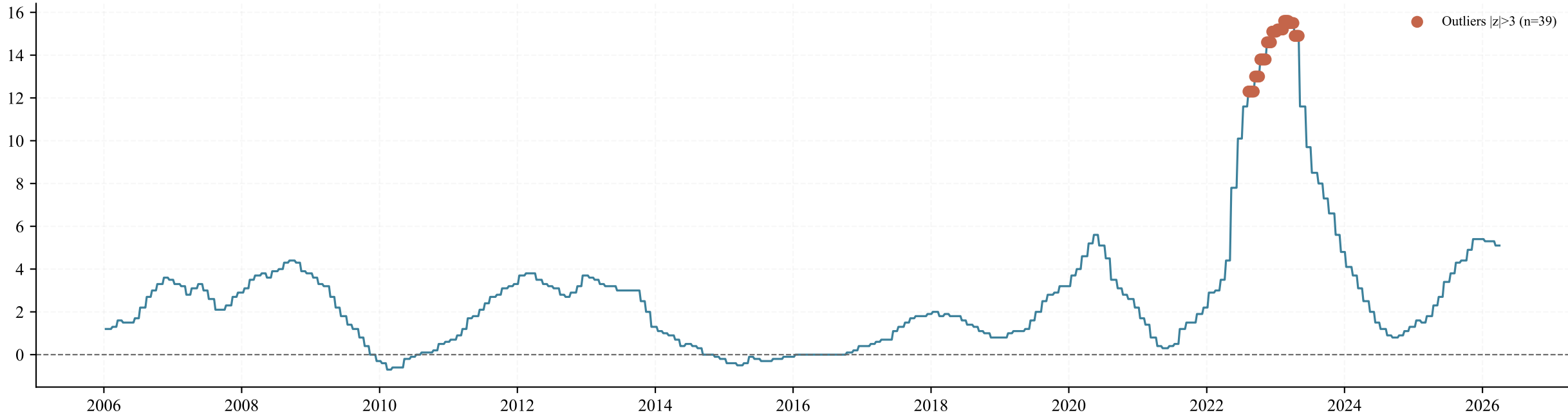
Time Series
