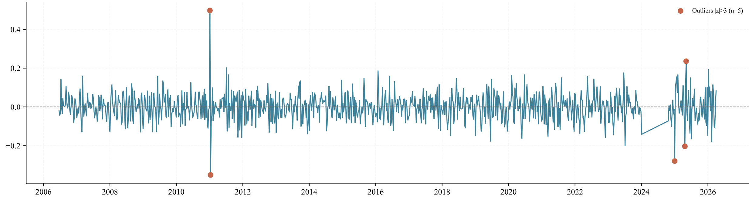
Time Series
