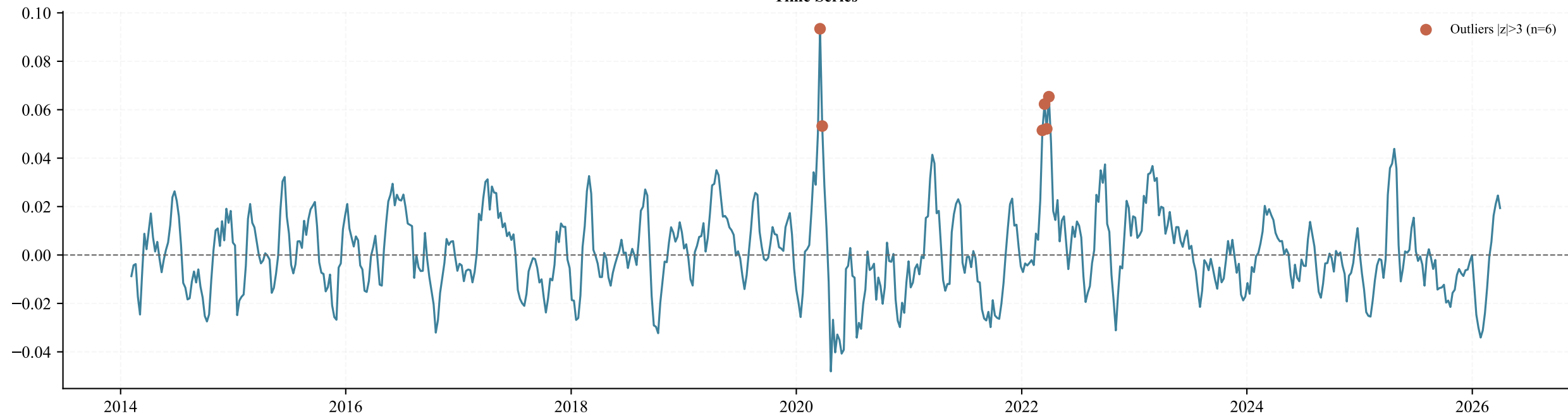
Time Series
