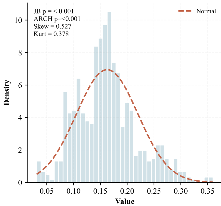
Distribution
