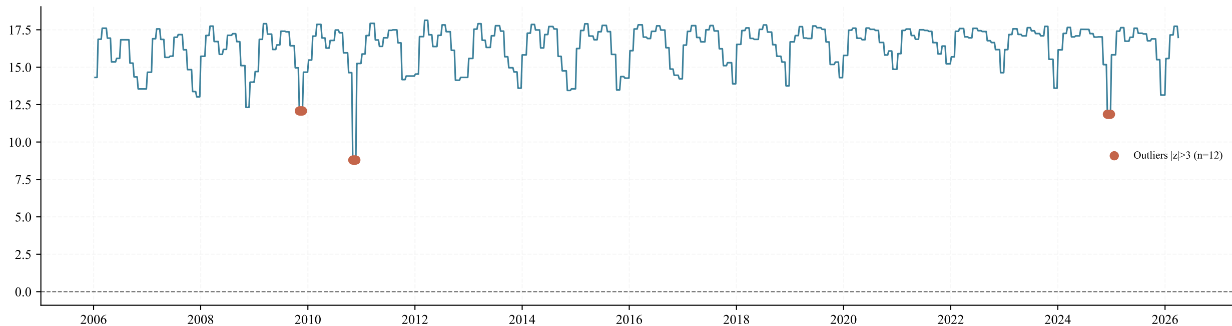
Time Series
