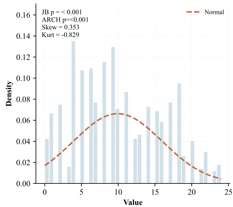
Distribution
