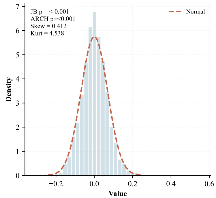
Distribution
