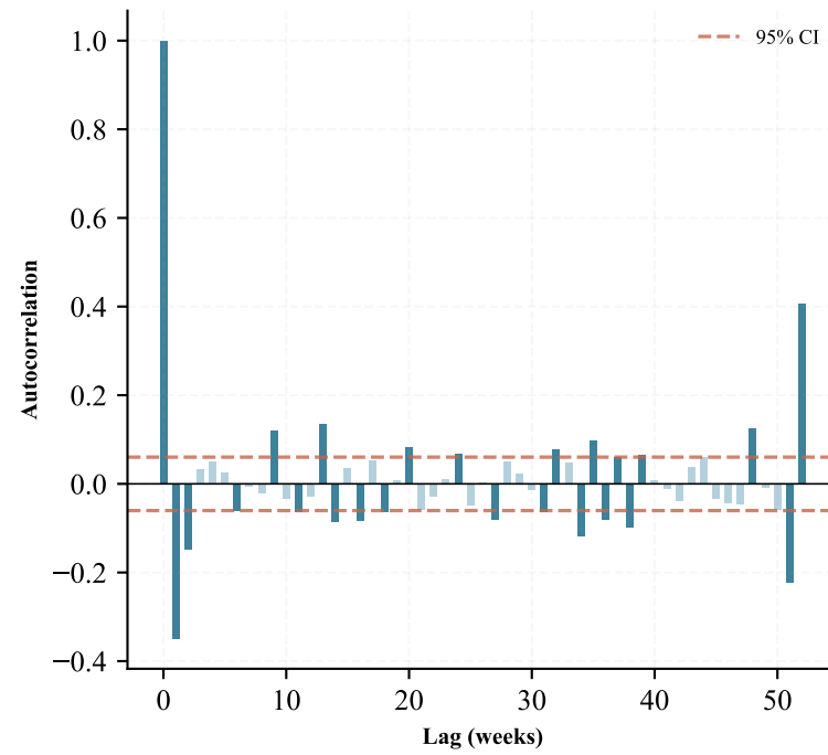
ACF ( \Delta Chilean Exports 1w)
