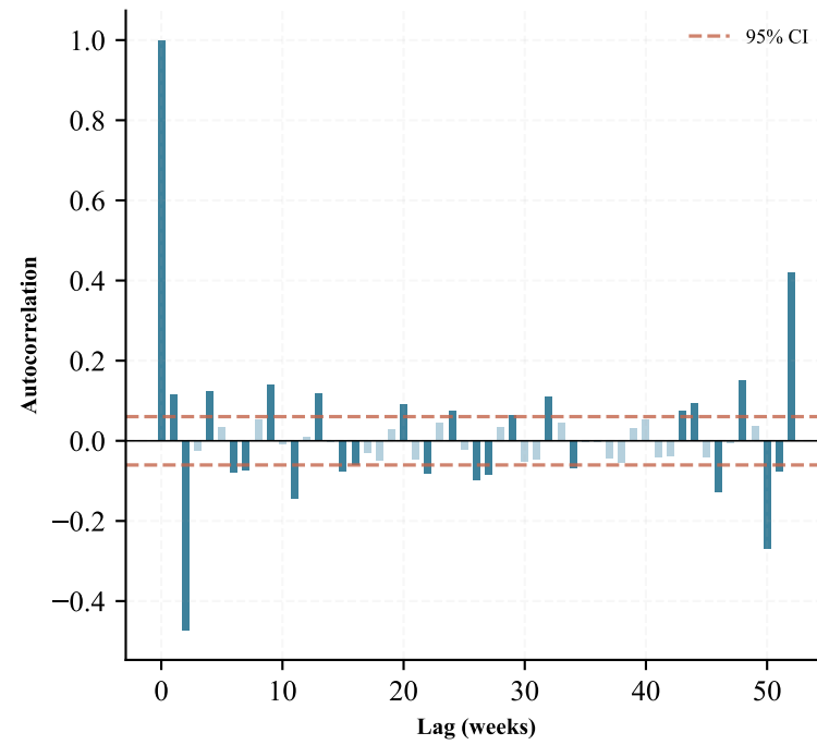
ACF ( \Delta Chilean Exports 2w)
