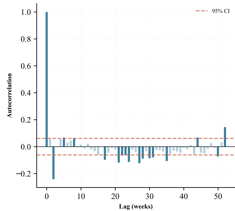
PACF ( \Delta FWD 6m)
