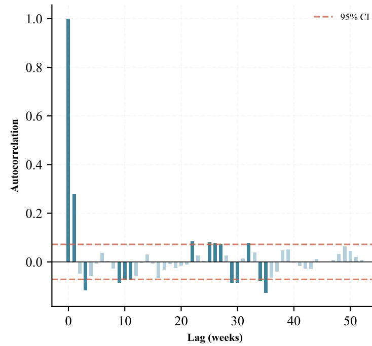
ACF ( \Delta Broiler Price (EU) 1w)
