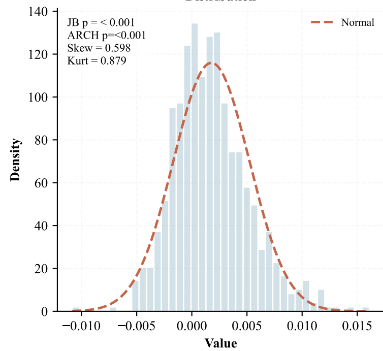
Distribution
