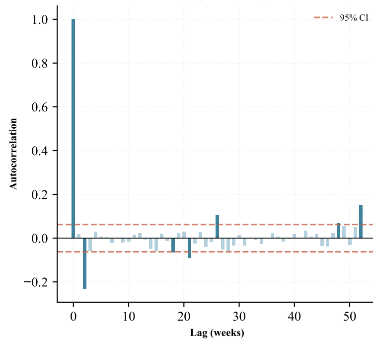
ACF ( \Delta FWD 12m)
