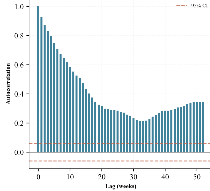
ACF (Soybean FWD Curvature)
