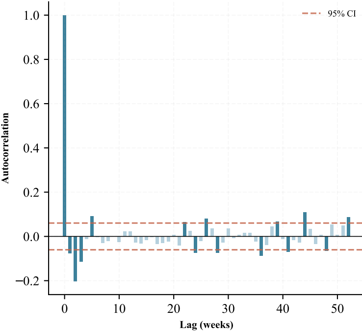
ACF ( \Delta Spread (FP - SSB))
