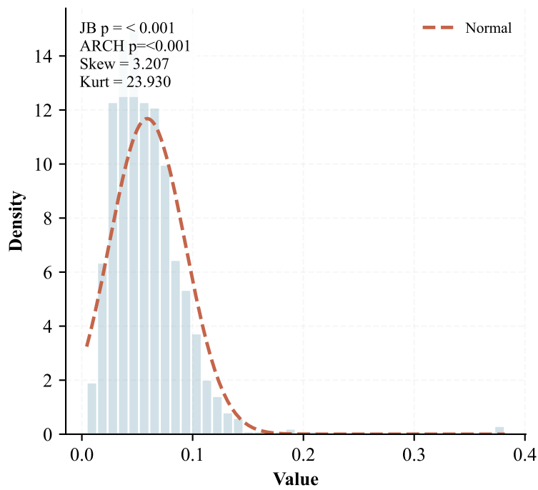
Distribution
