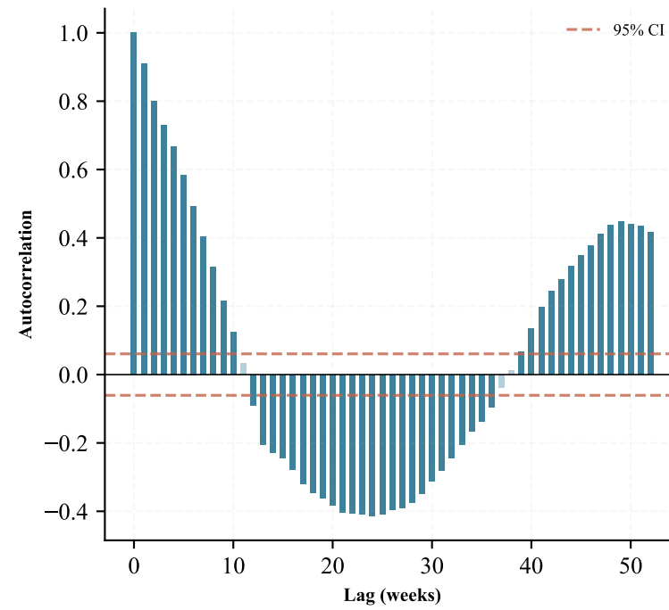
ACF ( \Delta Salmon (NOK/KG) 3m)
