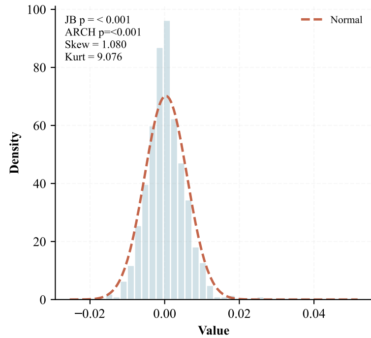
Distribution
