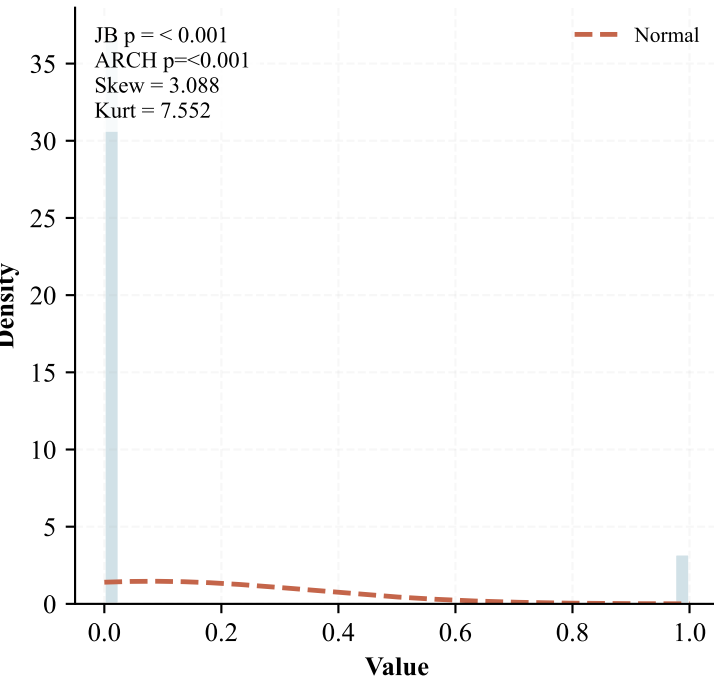
Distribution
