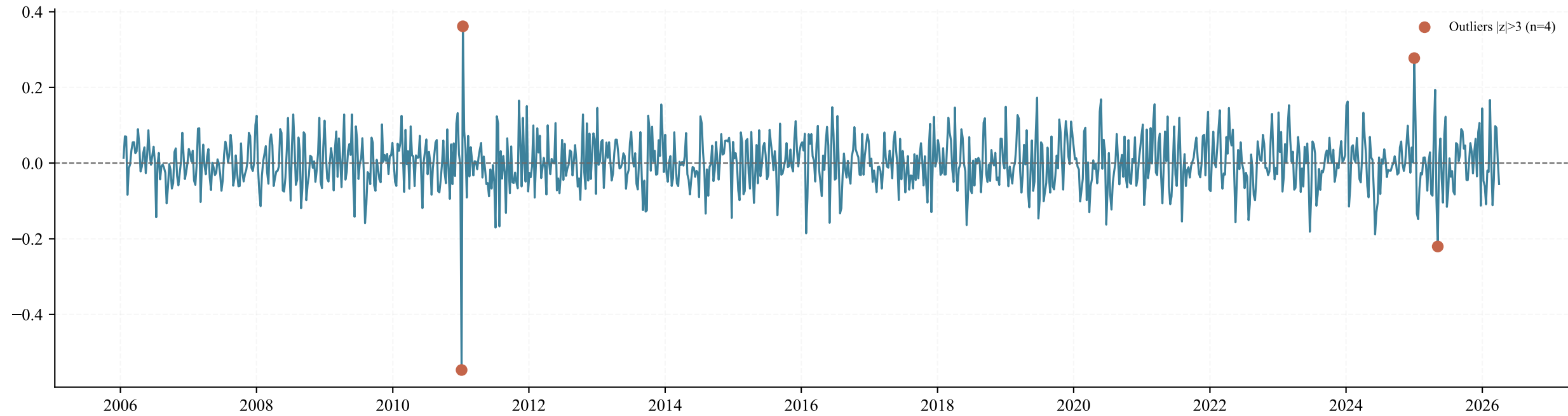
Time Series
