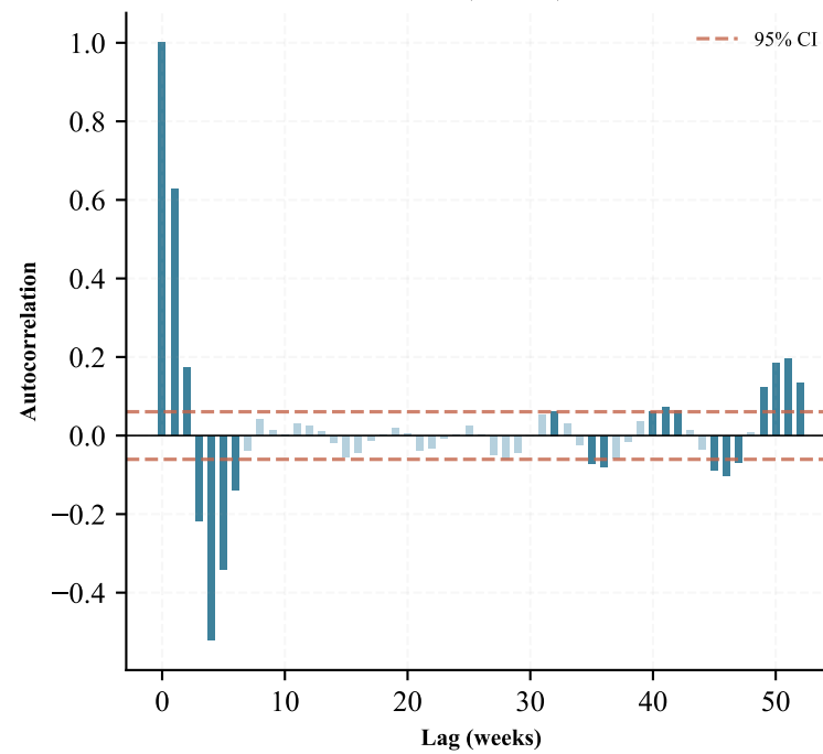
ACF (Acc 1m)
