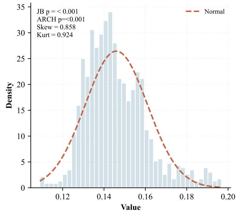
Distribution
