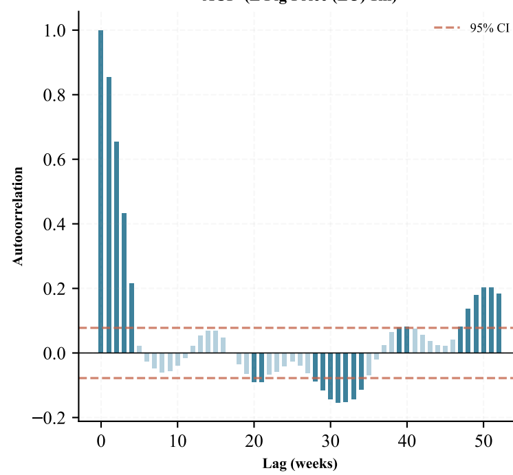
ACF ( \Delta Pig Price (EU) 1m)
