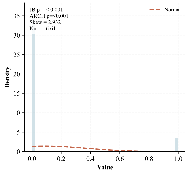
Distribution
