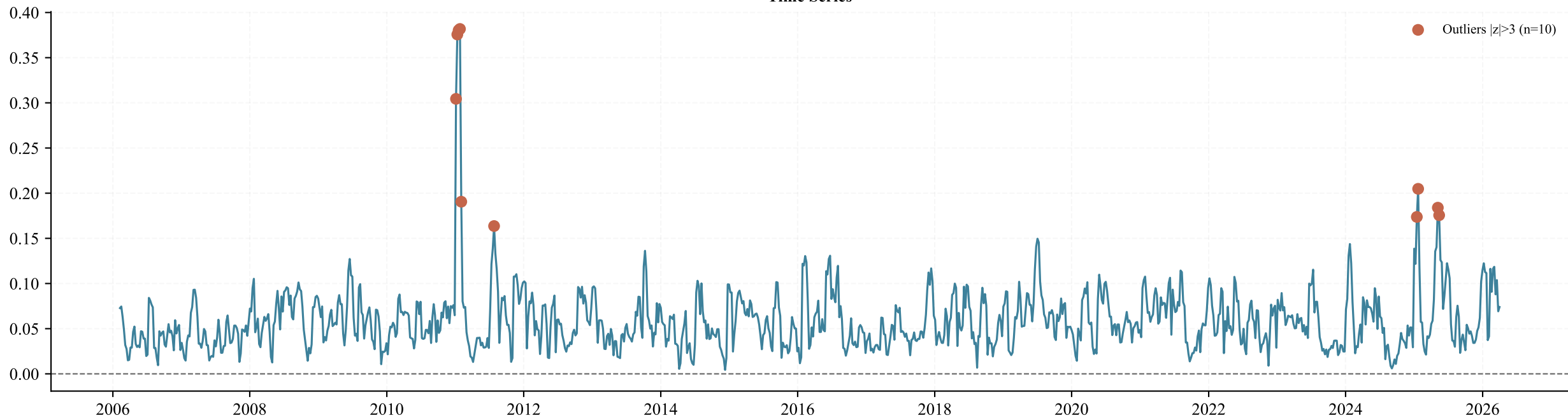
Time Series
