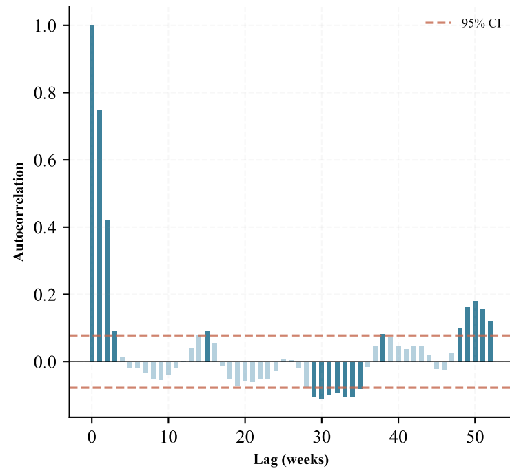
ACF ( \Delta Pig Price (EU) 2w)
