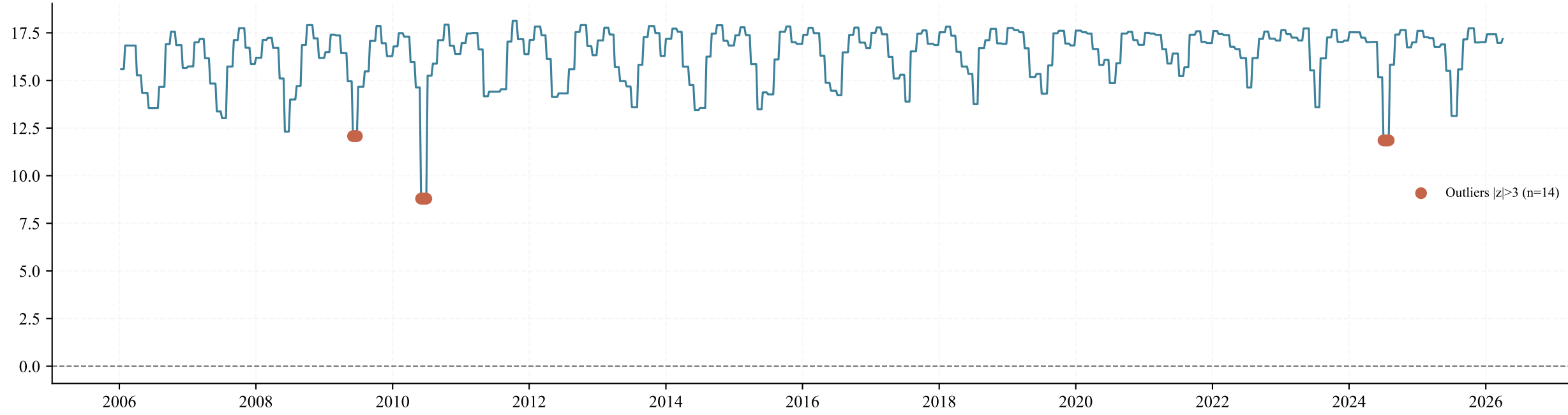
Time Series
