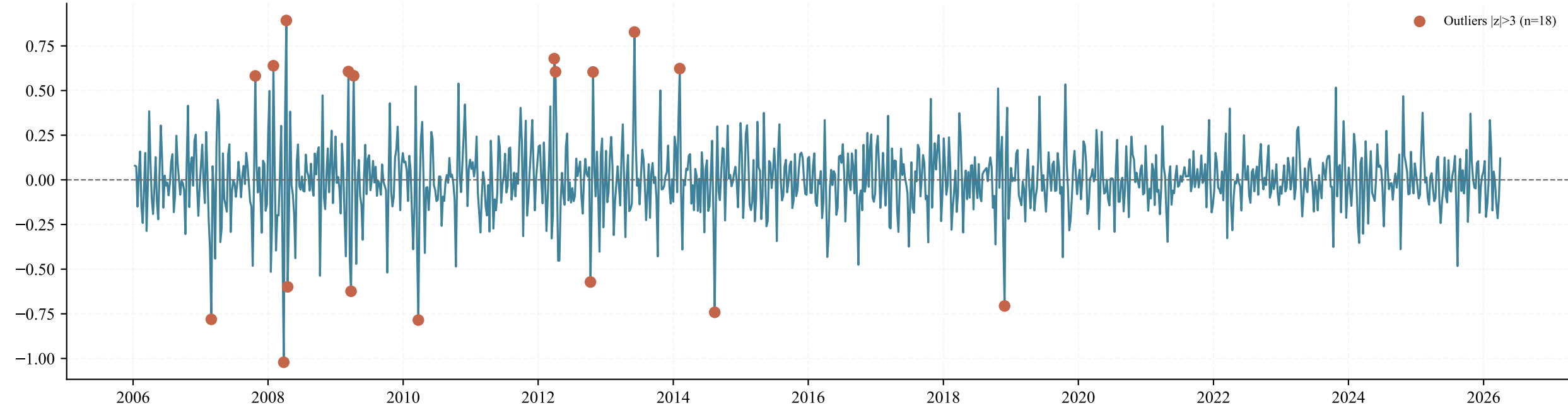
Time Series
