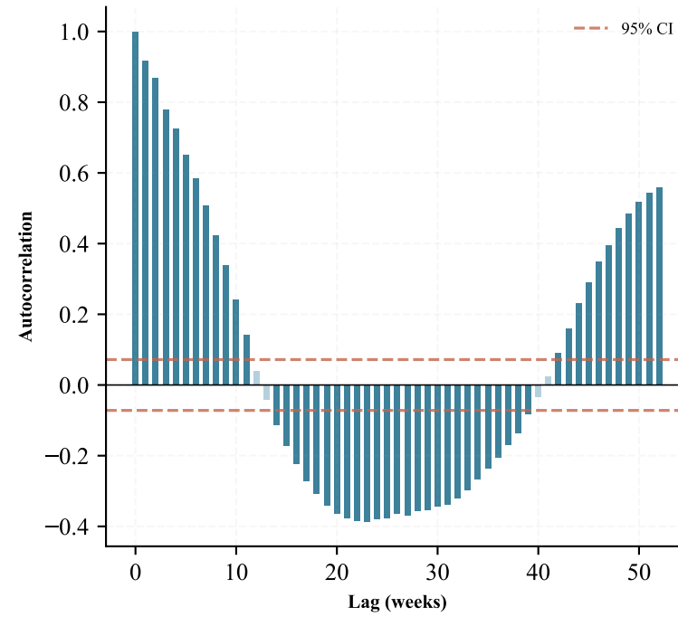
ACF (Lice Outbreak)
