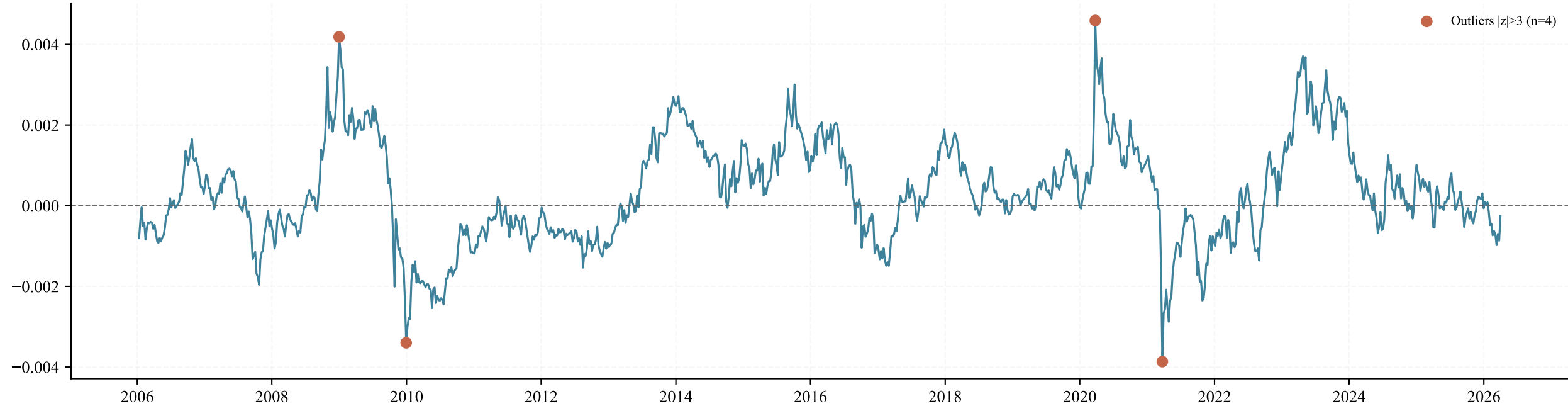
Time Series
