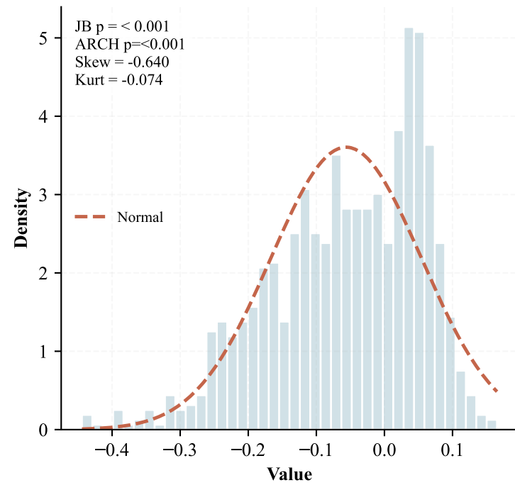
Distribution
