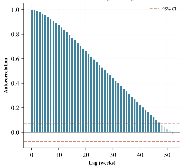
ACF (Sea Temp 12m Avg)
