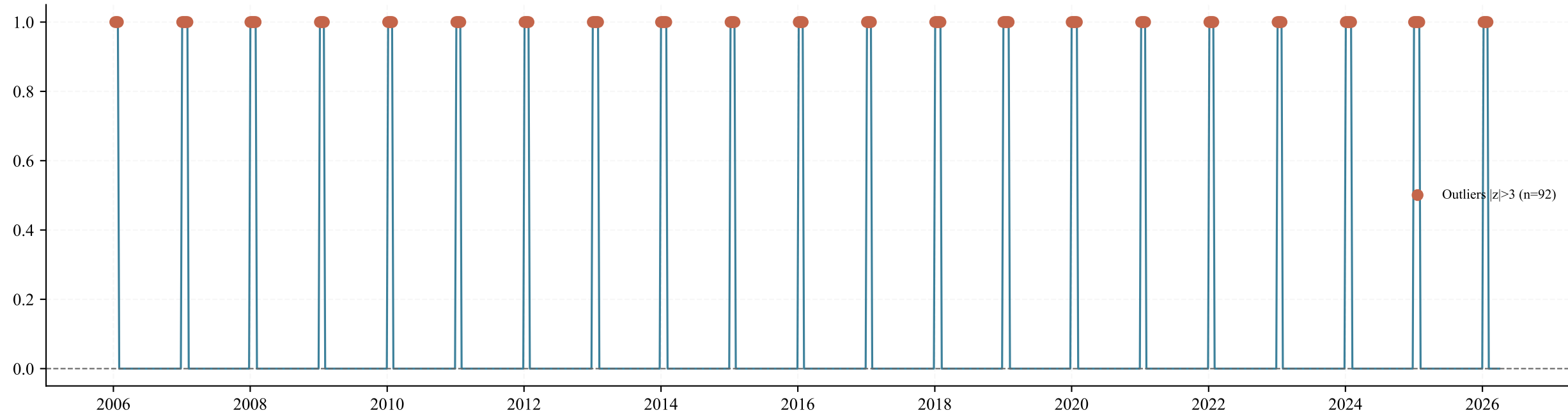
Time Series
