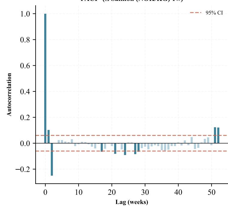
PACF ( \Delta Salmon (NOK/KG) 1w)
