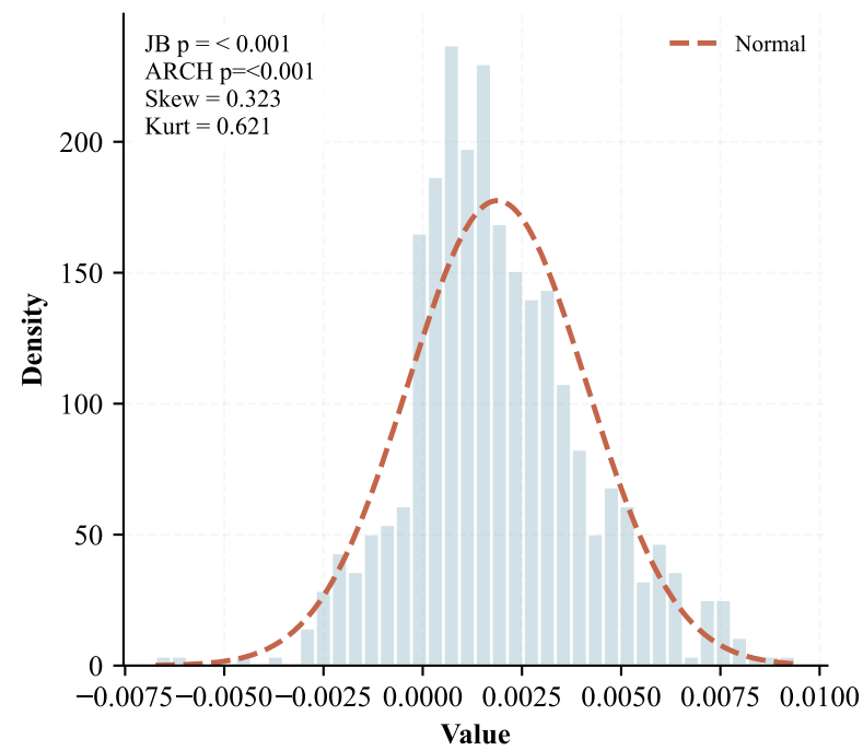
Distribution
