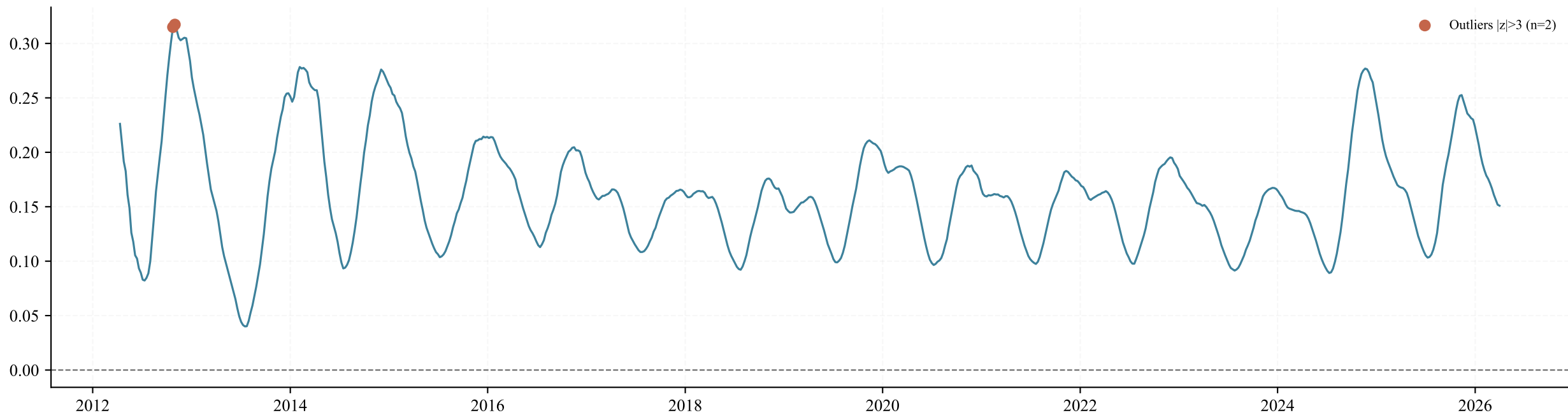
Time Series
