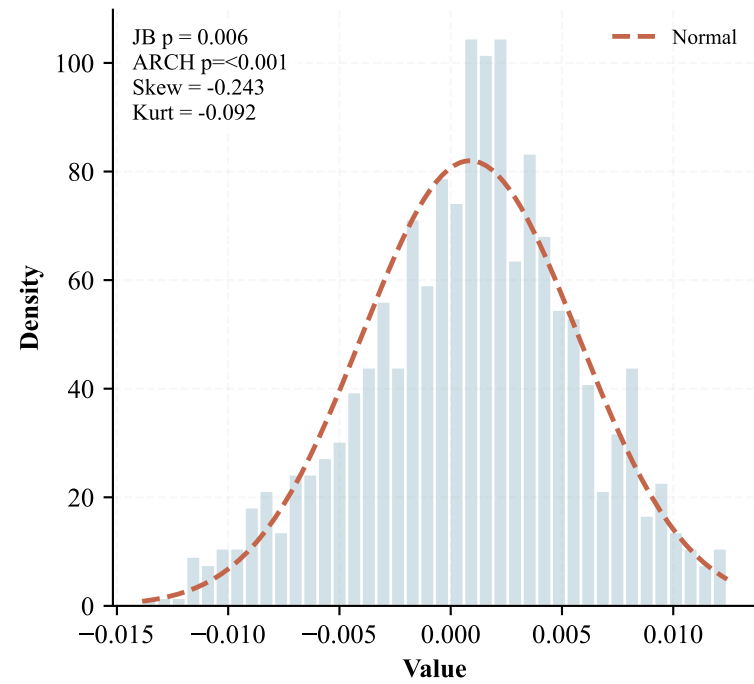
Distribution
