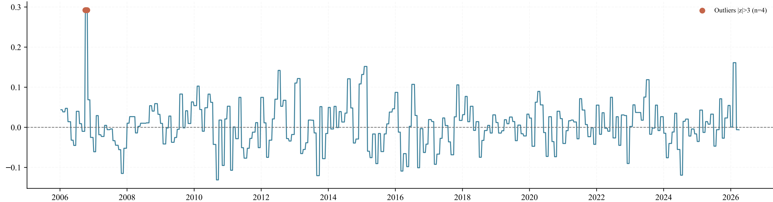
Time Series
