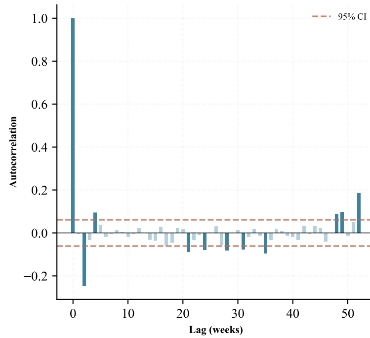
ACF ( \Delta FWD 3m)
