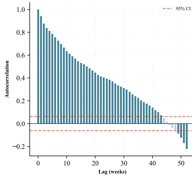
ACF ( \Delta Salmon (NOK/KG) 12m)
