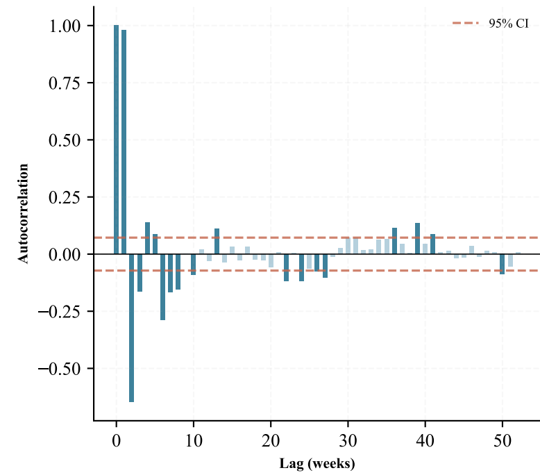
PACF (Lice Outbreak 1m)
