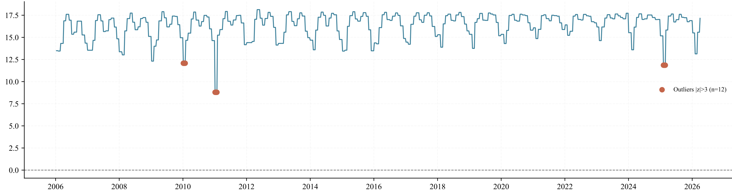
Time Series
