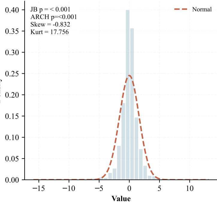
Distribution
