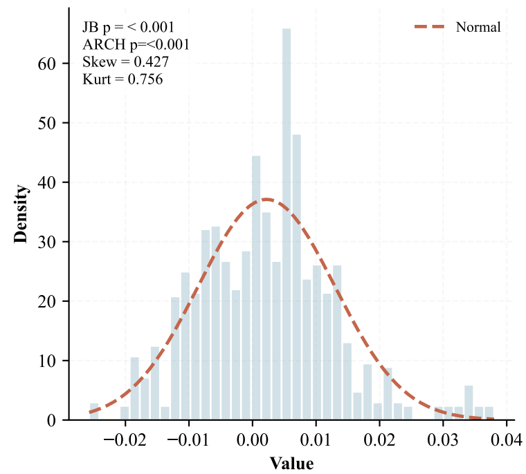
Distribution
