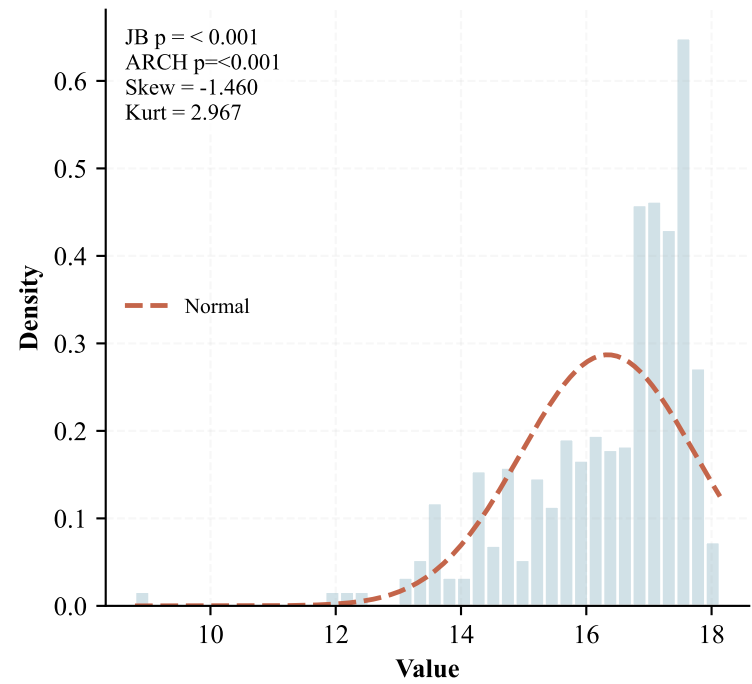
Distribution
