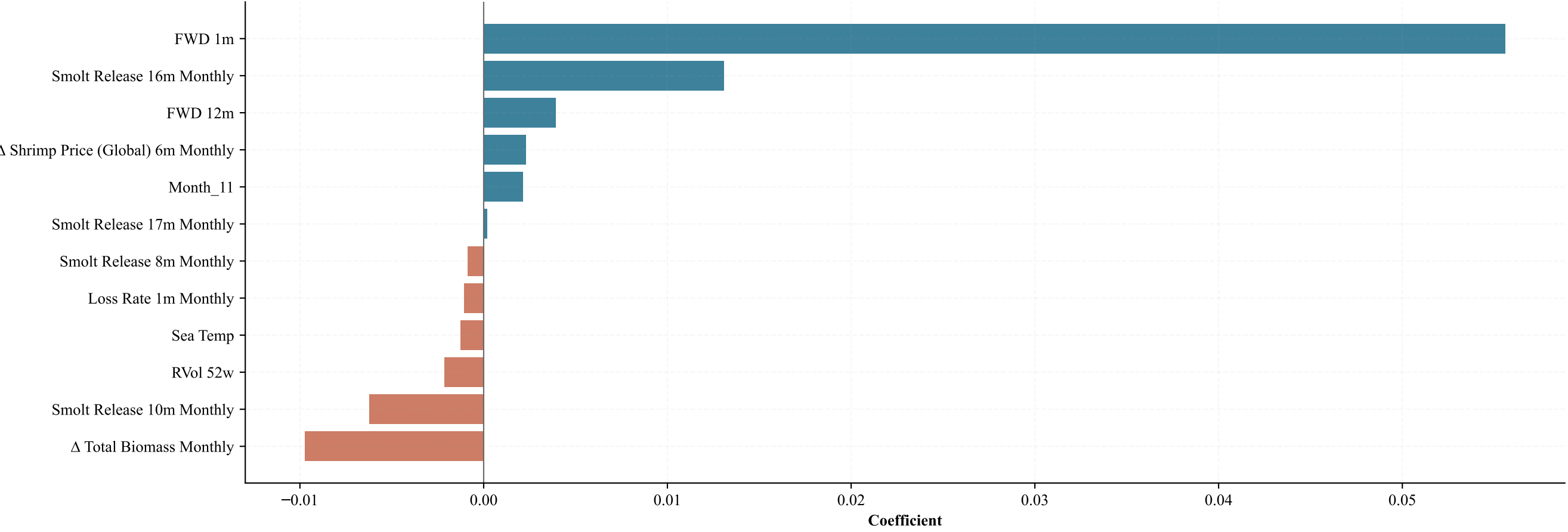
Non-zero Lasso Coefficients (12 selected, \alpha =0.01177)
