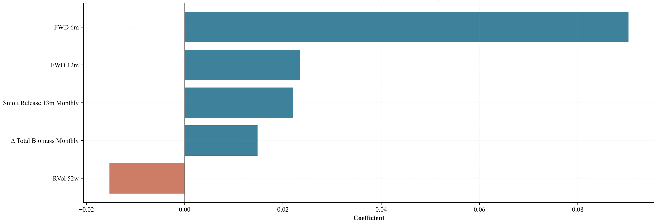
Non-zero Lasso Coefficients (5 selected, \alpha =0.03765)
