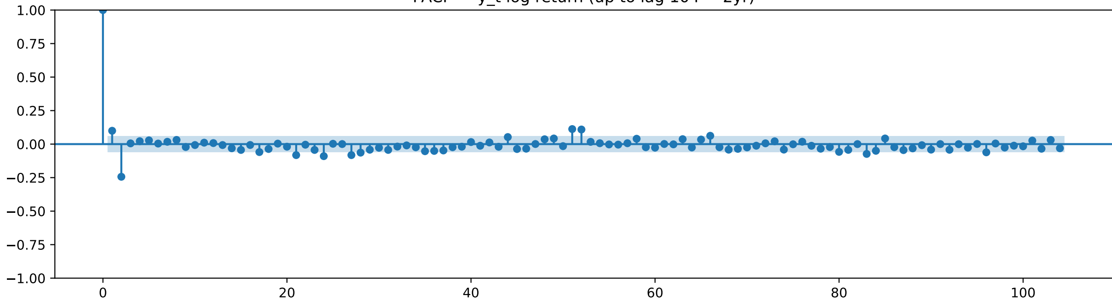
PACF — y_t log return (up to lag 104 = 2yr)
