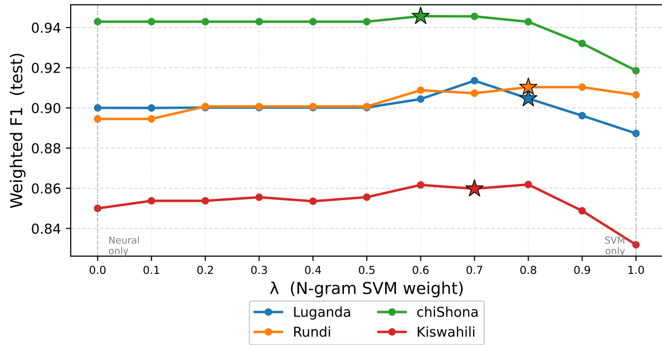
Hybrid interpolation sensitivity Best SVM + AfroXLMR (★ = best \lambda on validation set)
