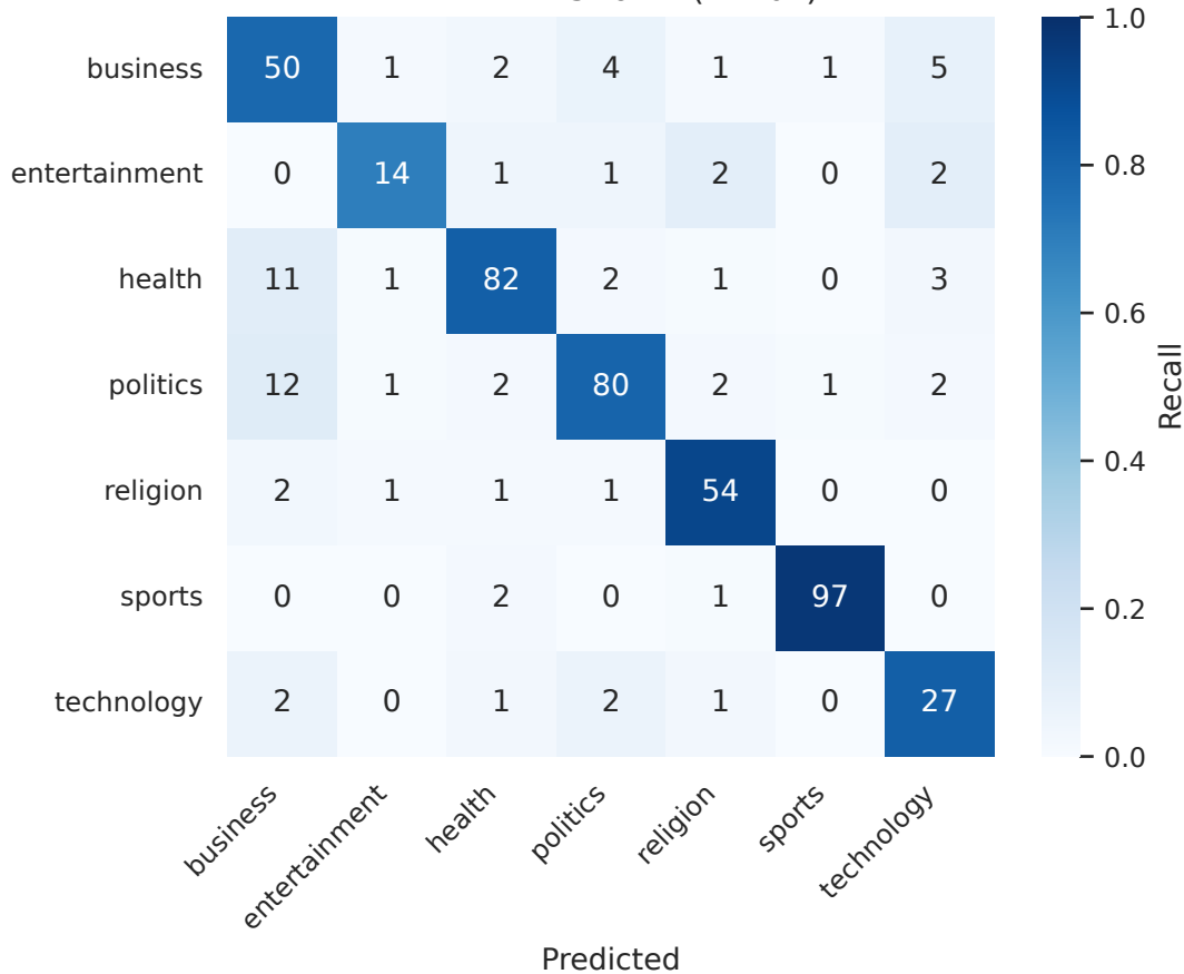
XLM-R - Kiswahili (N=full)
