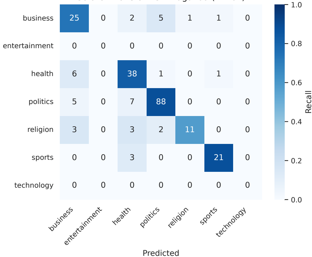
Scratch transformer - Luganda (N=full)
