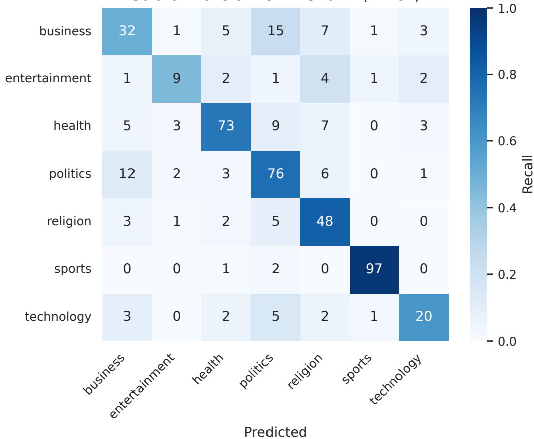
Scratch transformer - Kiswahili (N=full)
