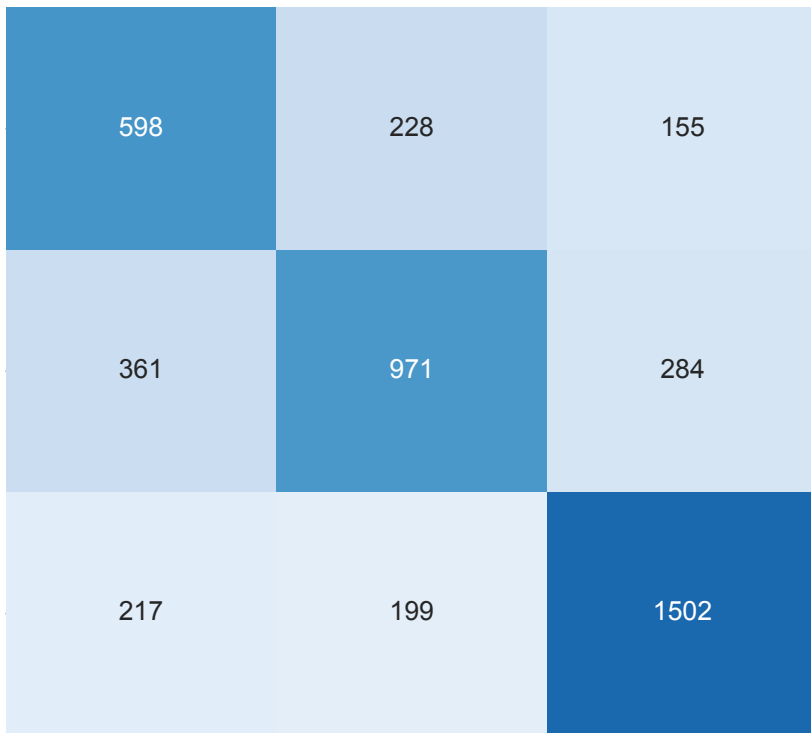
XLM-R - Yoruba (N=full)
