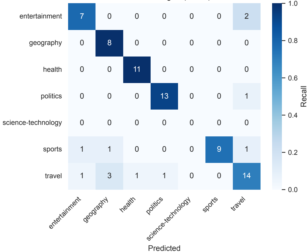
AfroXLMR - Igbo (N=full)
