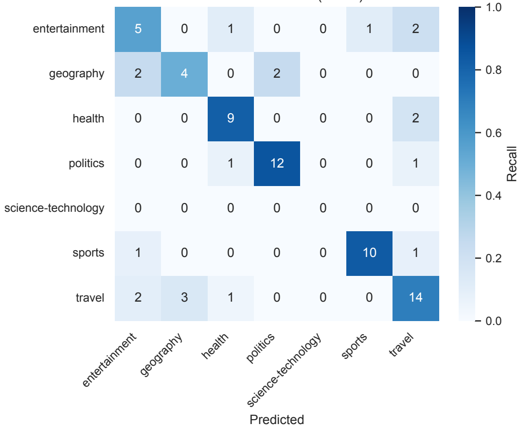
AfroXLMR - Yoruba (N=full)
