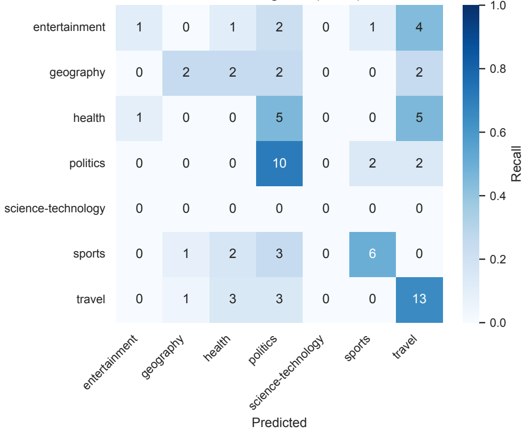
XLM-R - Luganda (N=full)
