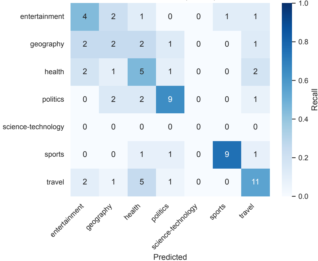
XLM-R - Rundi (N=500)
