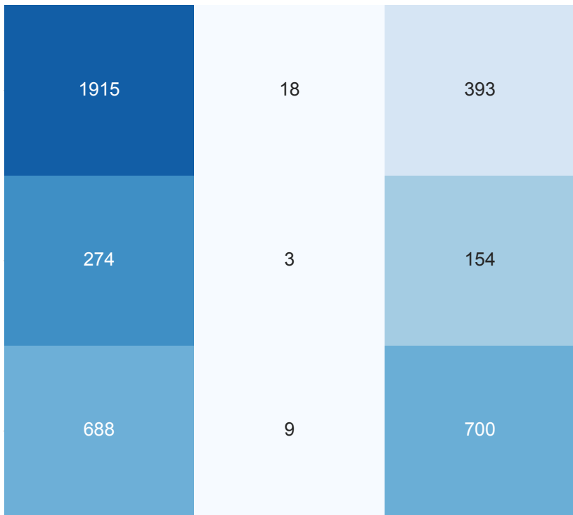
Scratch transformer - Nig. Pidgin (N=full)
