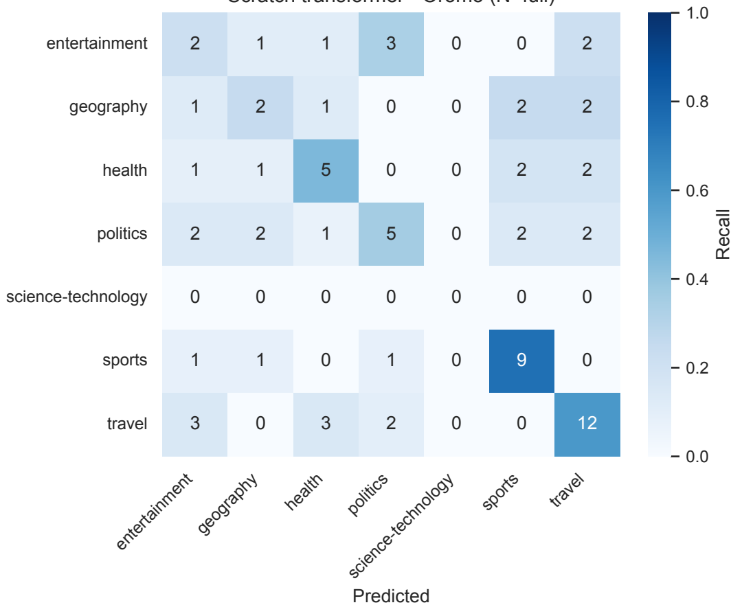
Scratch transformer - Oromo (N=full)
