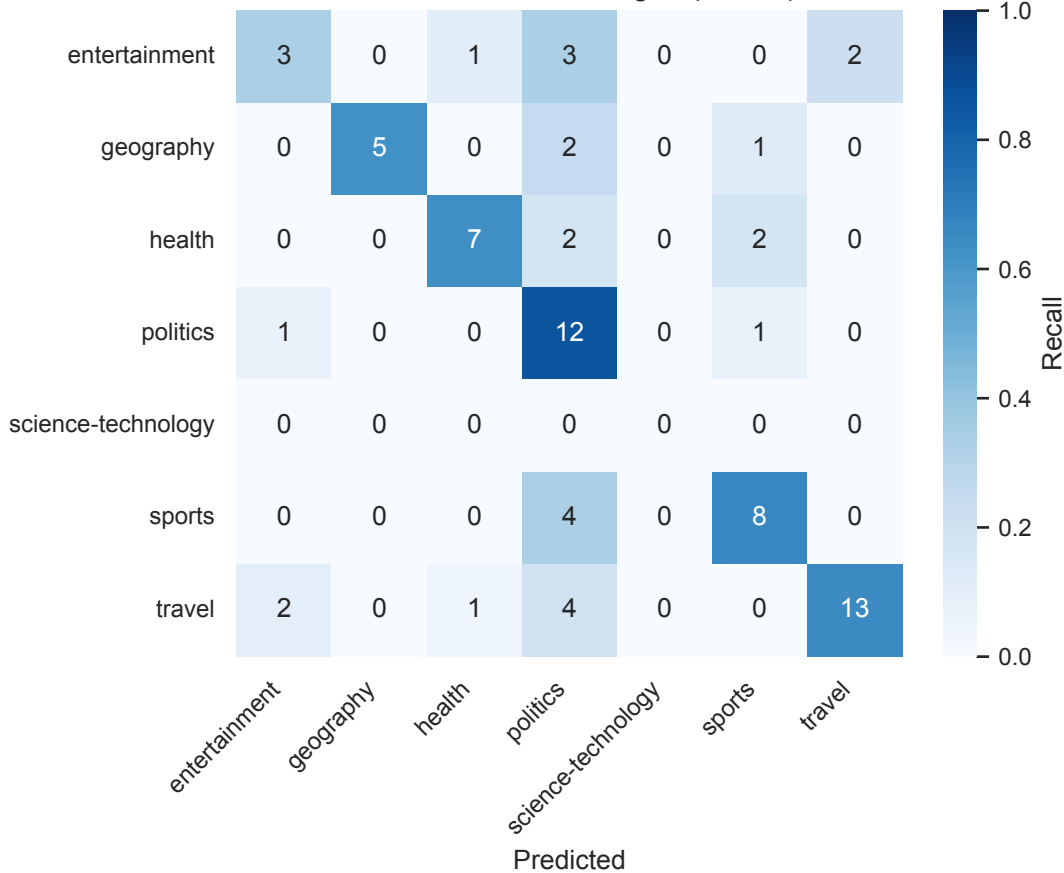
Scratch transformer - Igbo (N=500)
