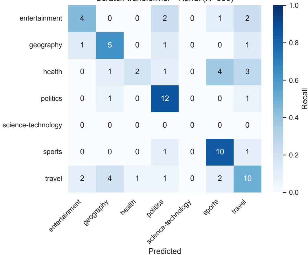
Scratch transformer - Rundi (N=500)
