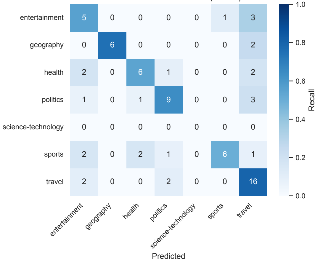
Scratch transformer - Swahili (N=500)
