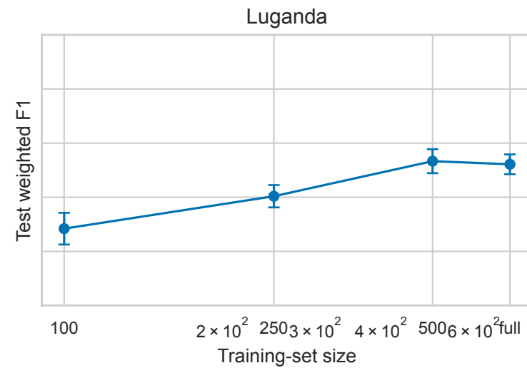
Scratch transformer: test weighted F1 vs training-set size (SIB-200)
