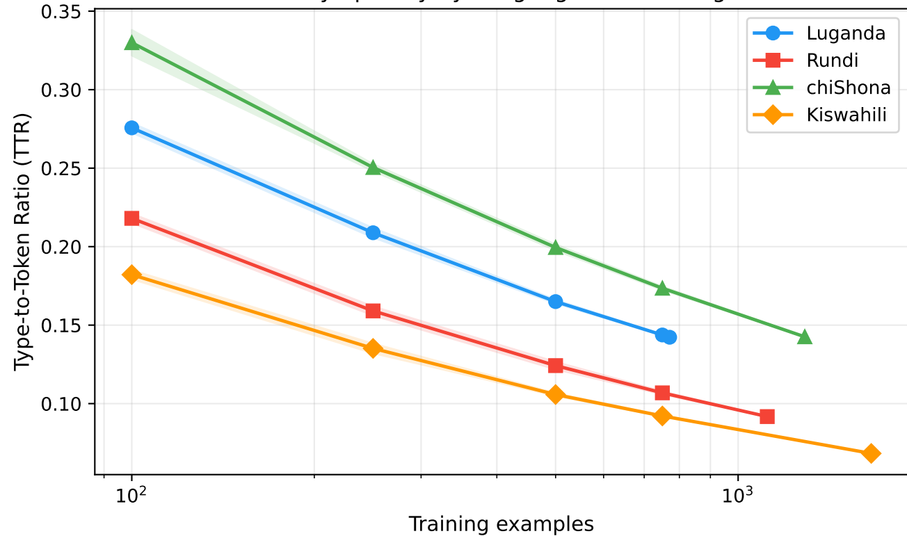
Vocabulary Sparsity by Language and Training Scale
