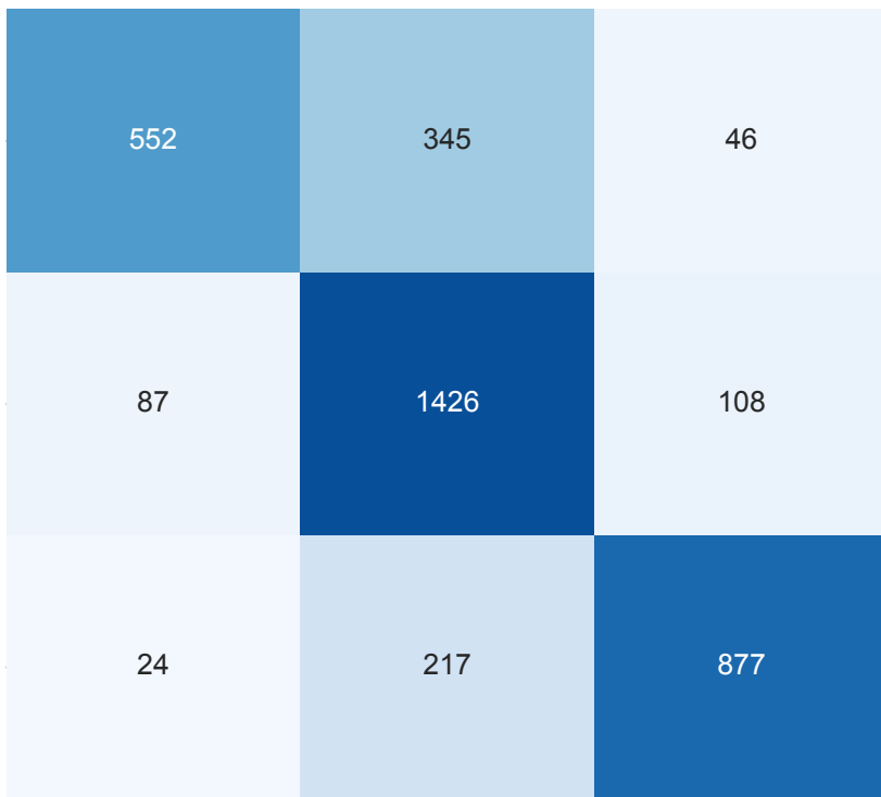
XLM-R - Igbo (N=full)
