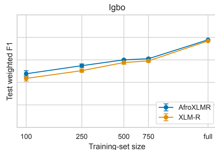
Test weighted F1 vs training-set size
