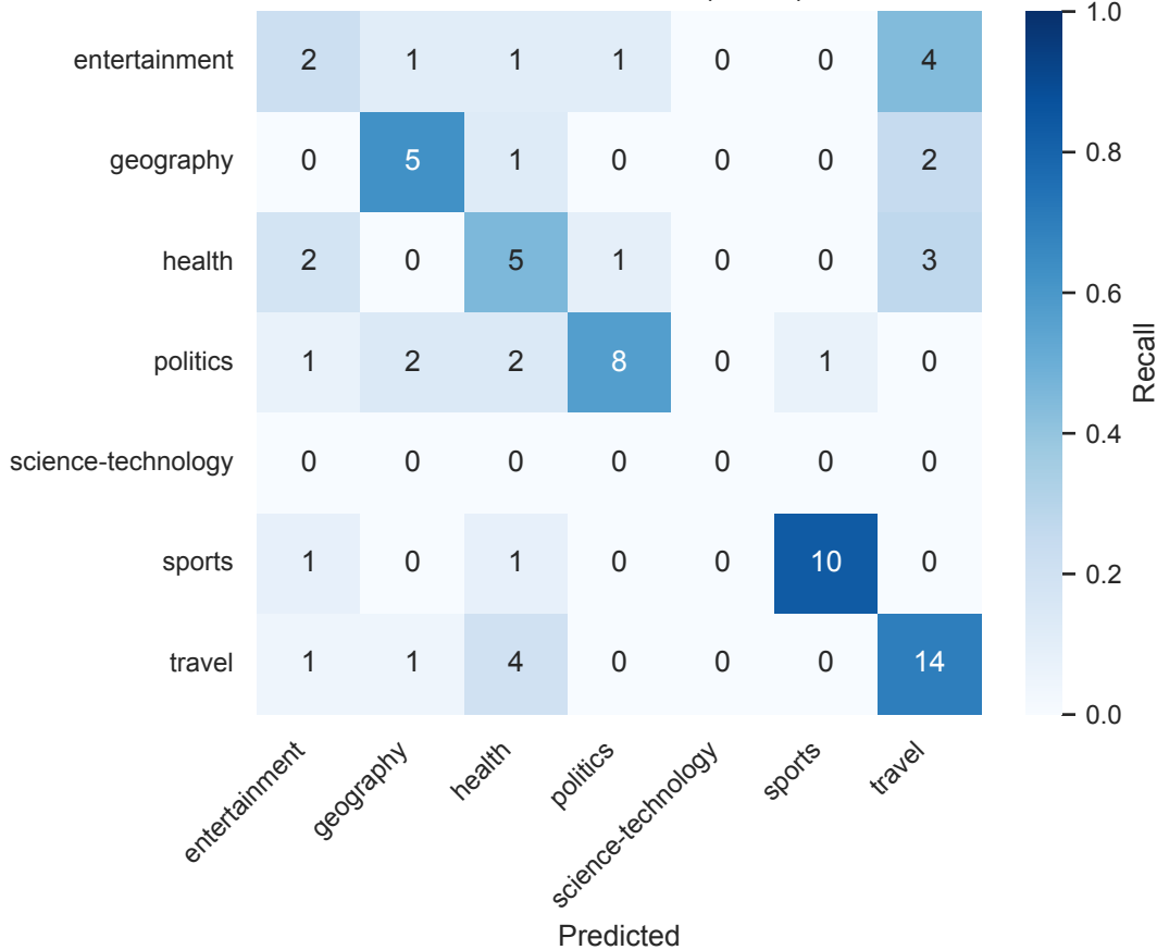
XLM-R - chiShona (N=full)
