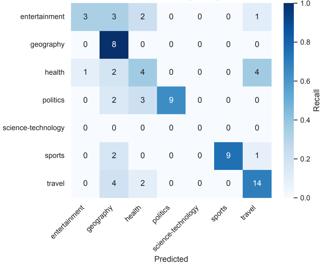
XLM-R - Yoruba (N=500)
