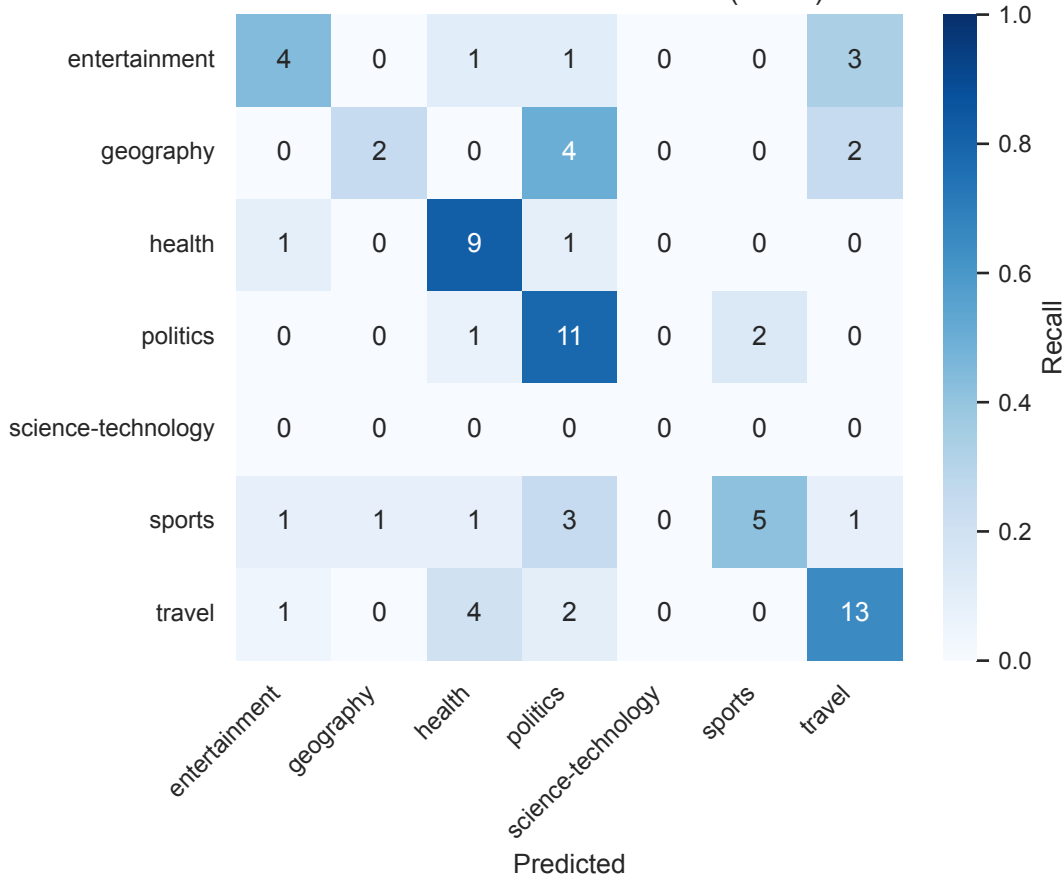
Scratch transformer - chiShona (N=full)
