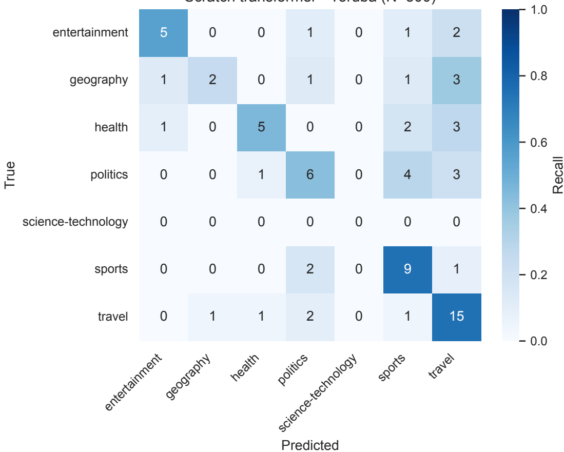
Scratch transformer - Yoruba (N=500)
