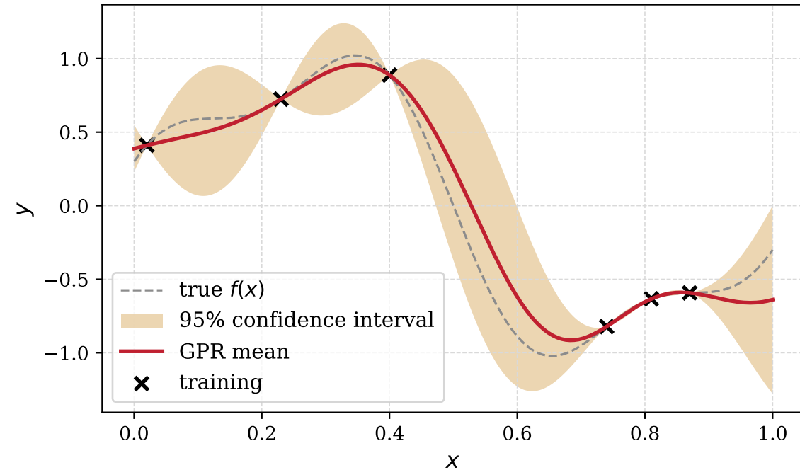
GPR (probabilistic)
