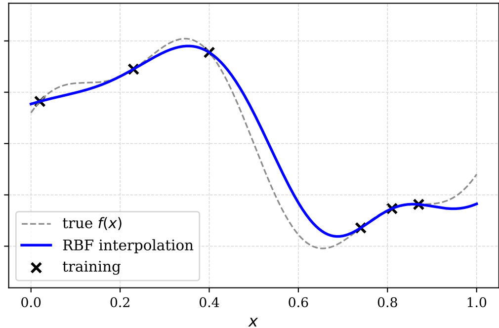
RBF (deterministic)
