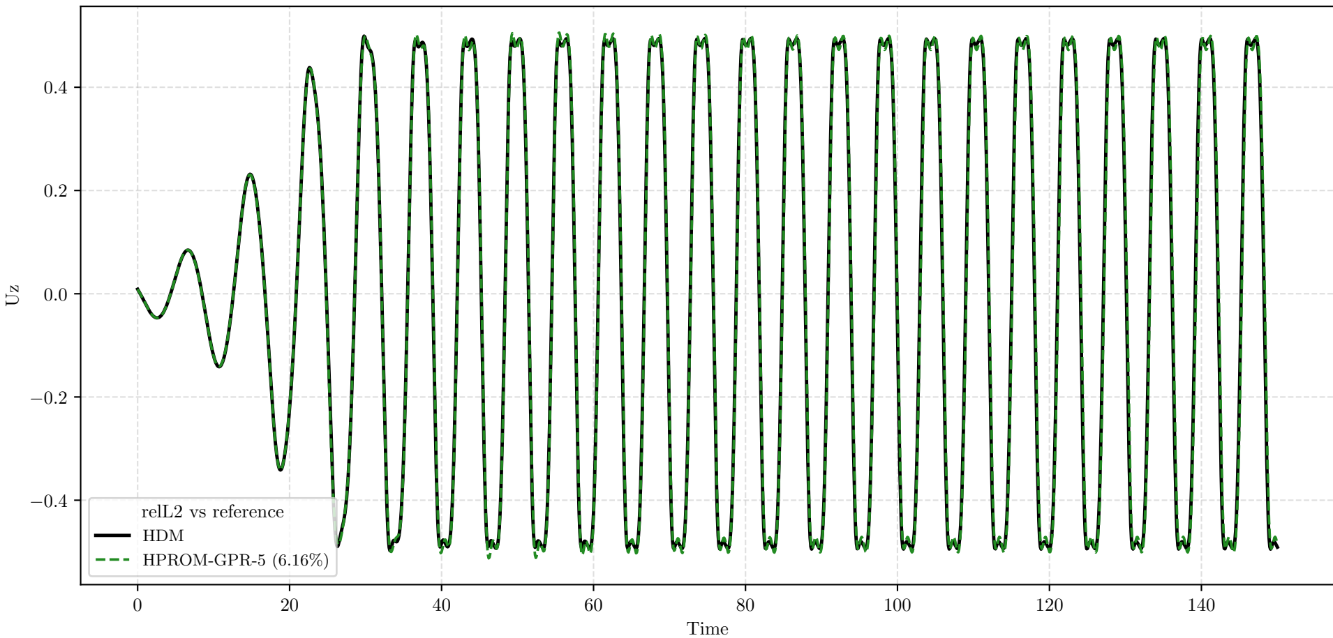
Probe Velocity Z
