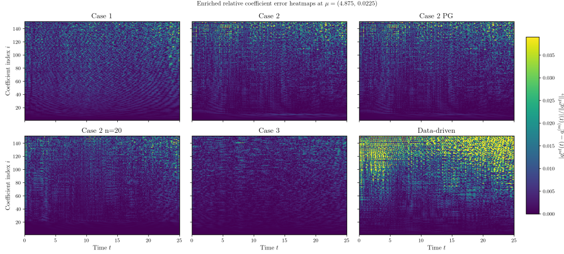
Figure 16: Enriched stage: relative coefficient error heatmaps at \mu^{(v)} for all available enriched models.
