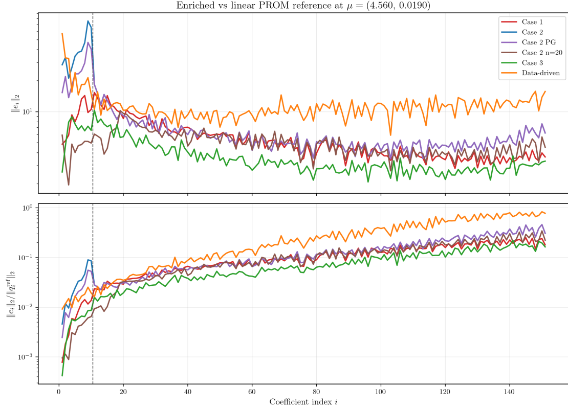
Figure 8: Enriched stage: per-index absolute and relative coefficient errors at \boldsymbol{\mu}^{(1)} = (4.56, 0.019) , including Case 2 PG Oracle and Case 2 n = 20 (native).
