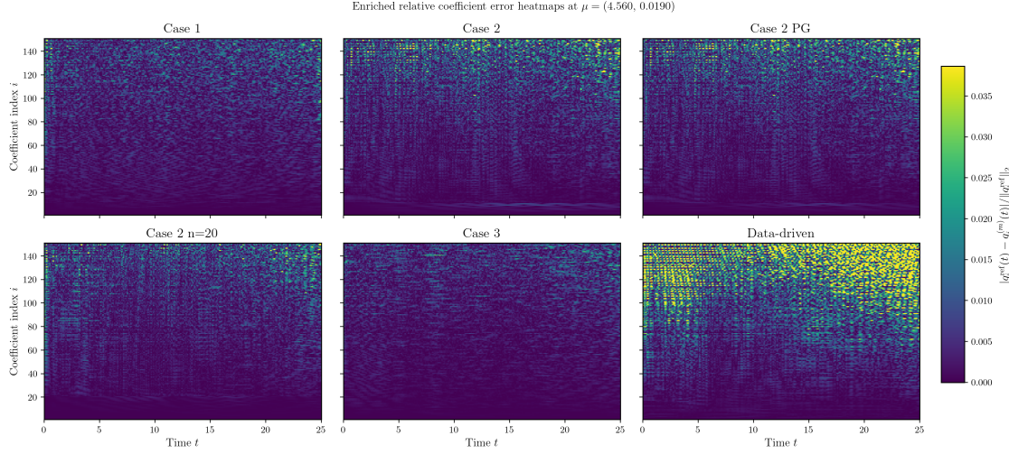
Figure 20: Enriched stage: relative coefficient error heatmaps at \mu^{(1)} = (4.56, 0.019) for all available enriched models.
