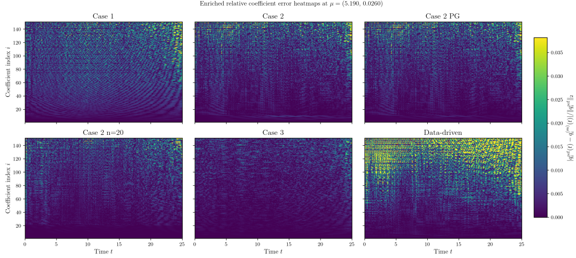
Figure 24: Enriched stage: relative coefficient error heatmaps at \mu^{(2)} = (5.19, 0.026) for all available enriched models.
