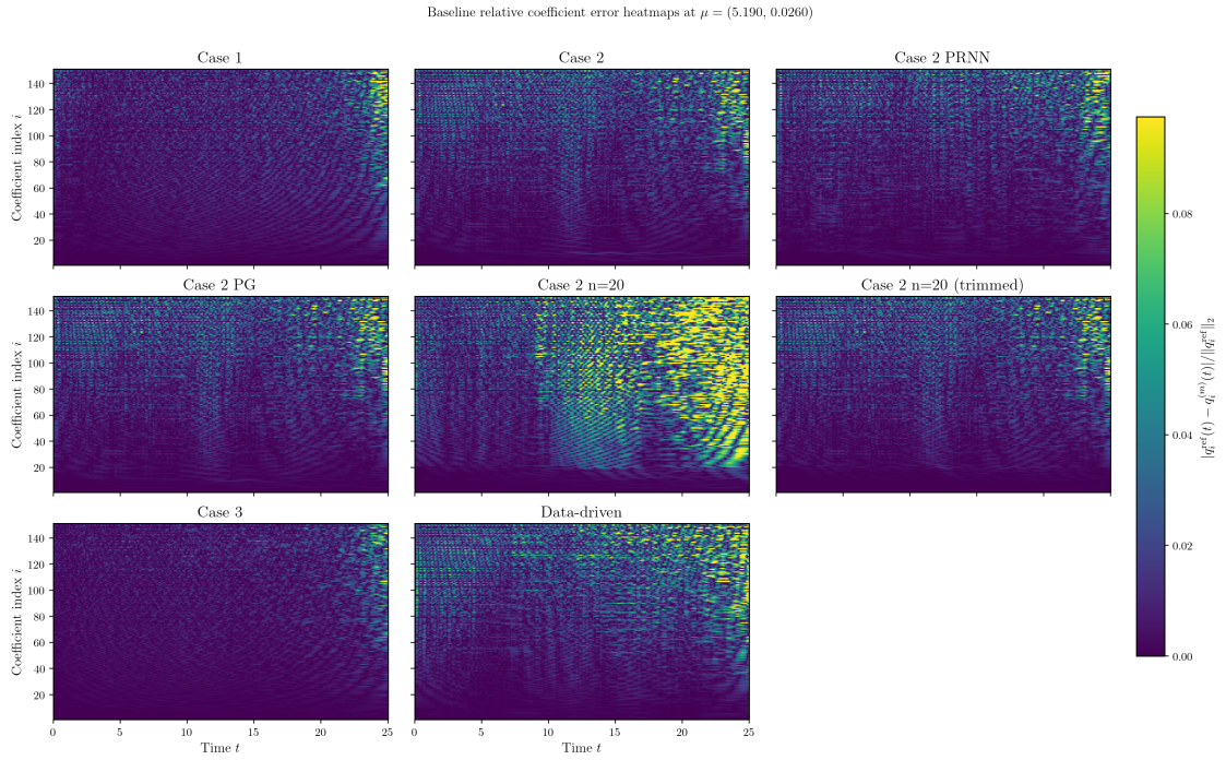
Figure 22: Baseline stage: relative coefficient error heatmaps at \mu^{(2)} = (5.19, 0.026) for all available baseline models.
