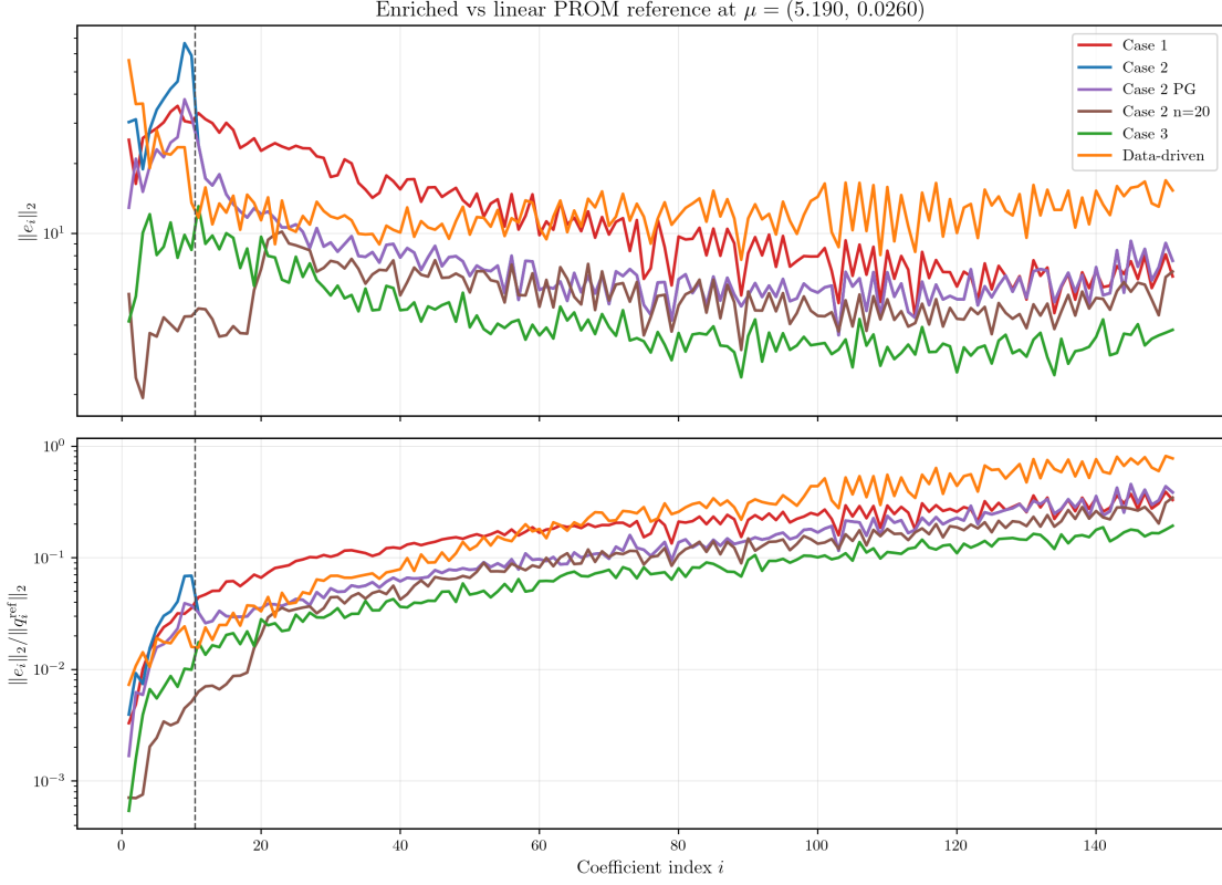
Figure 10: Enriched stage: per-index absolute and relative coefficient errors at \boldsymbol{\mu}^{(2)} = (5.19, 0.026) , including Case 2 PG Oracle and Case 2 n = 20 (native).
