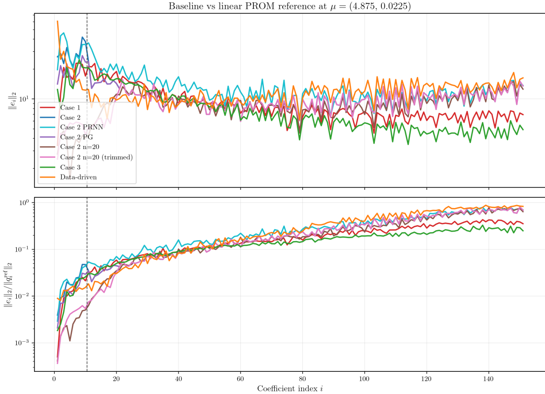
Figure 5: Baseline stage: per-index absolute and relative coefficient errors vs linear n_{\text{tot}} -PROM reference at \boldsymbol{\mu}^{(v)} = (4.875, 0.0225) , including Case 2 PRNN, Case 2 PG Oracle, Case 2 n = 20 (native), and Case 2 n = 20 (trimmed transfer).
