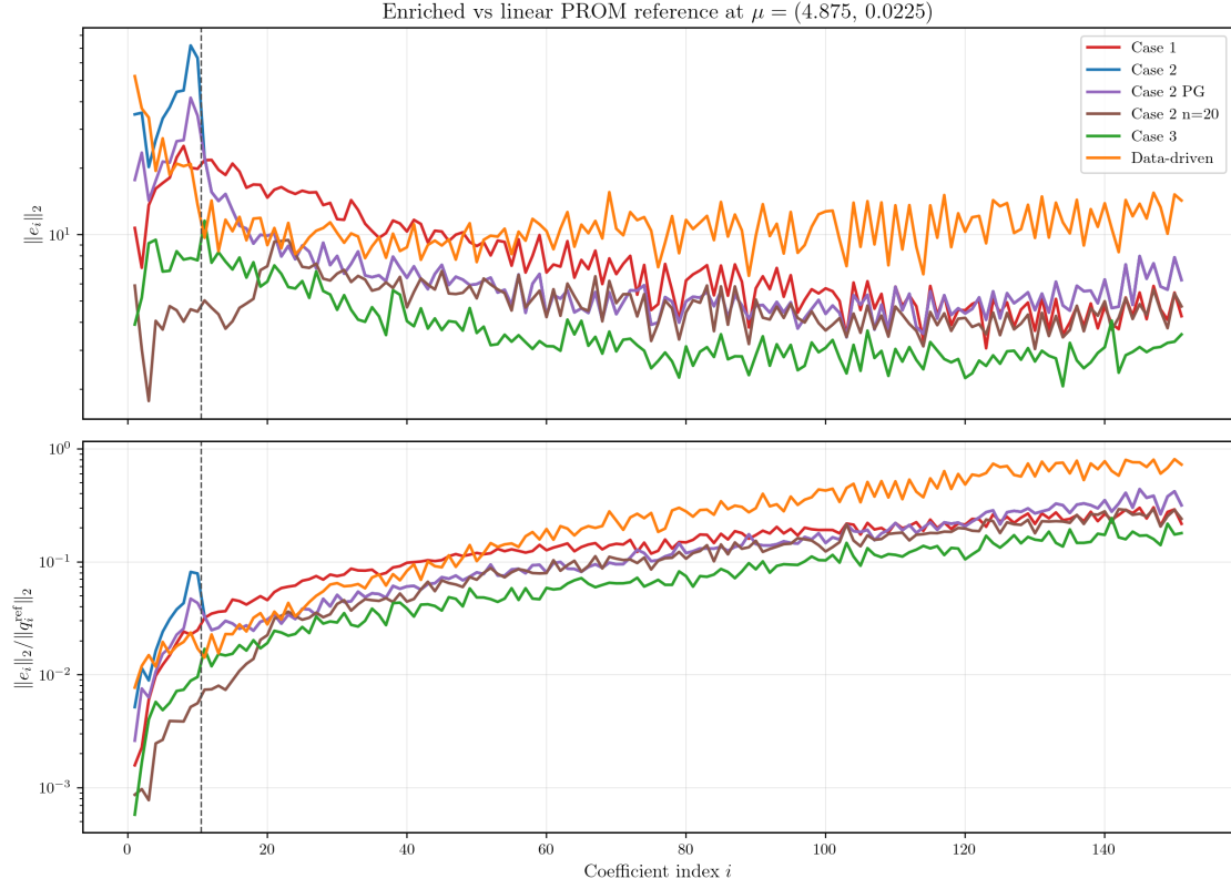
Figure 6: Enriched stage: per-index absolute and relative coefficient errors vs linear n_{\text{tot}} -PROM reference at \mu^{(v)} = (4.875, 0.0225) , including Case 2 PG Oracle and Case 2 n = 20 (native).
