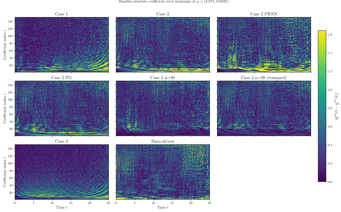
Figure 13: Baseline stage: absolute coefficient error heatmaps \left|q_i^{\text{ref}}(t) - q_i^{(m)}(t)\right| for all available baseline models.
