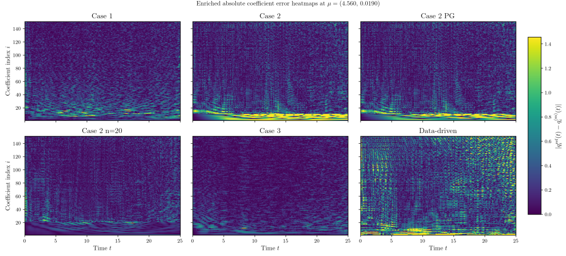
Figure 19: Enriched stage: absolute coefficient error heatmaps at \mu^{(1)} = (4.56, 0.019) for all available enriched models.
