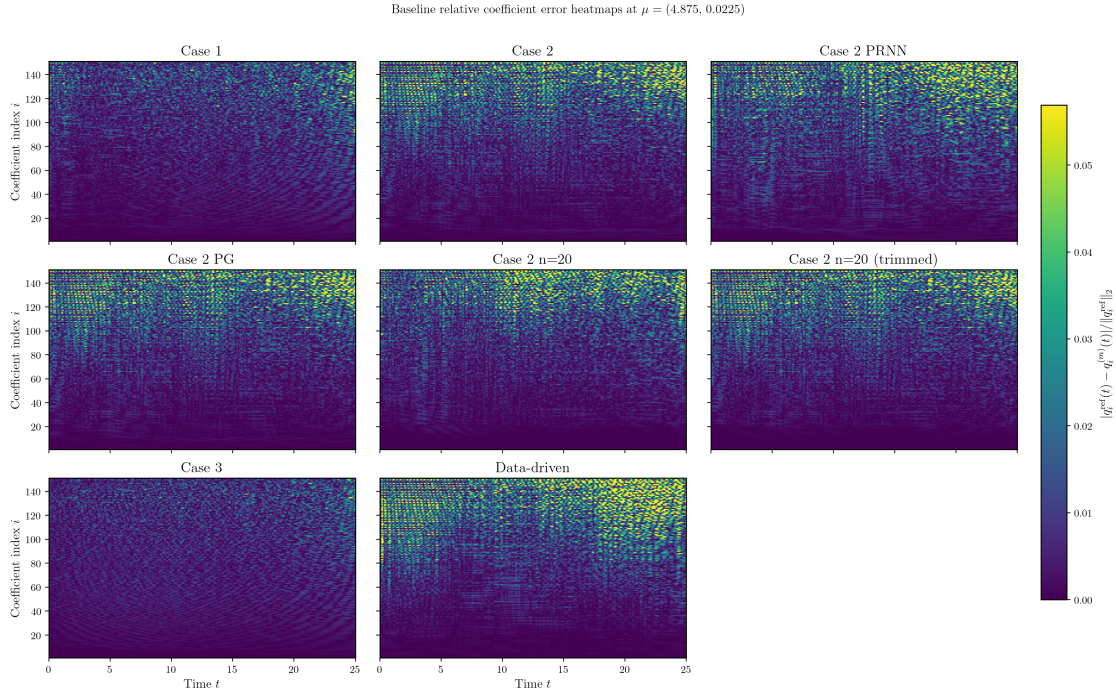
Figure 14: Baseline stage: relative coefficient error heatmaps for all available baseline models, using normalization by \|q_i^{\text{ref}}\|_2 .
