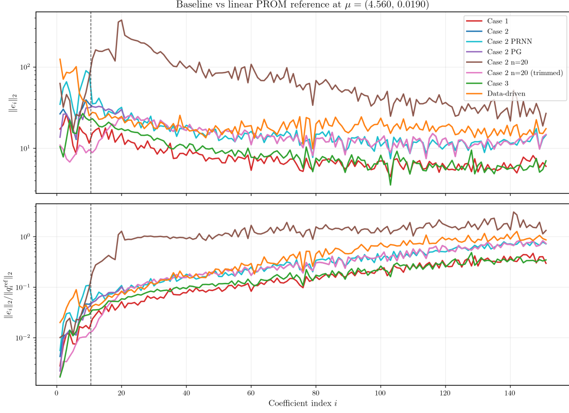
Figure 7: Baseline stage: per-index absolute and relative coefficient errors at \mu^{(1)} = (4.56, 0.019) , including Case 2 PRNN, Case 2 PG Oracle, Case 2 n = 20 (native), and Case 2 n = 20 (trimmed transfer).
