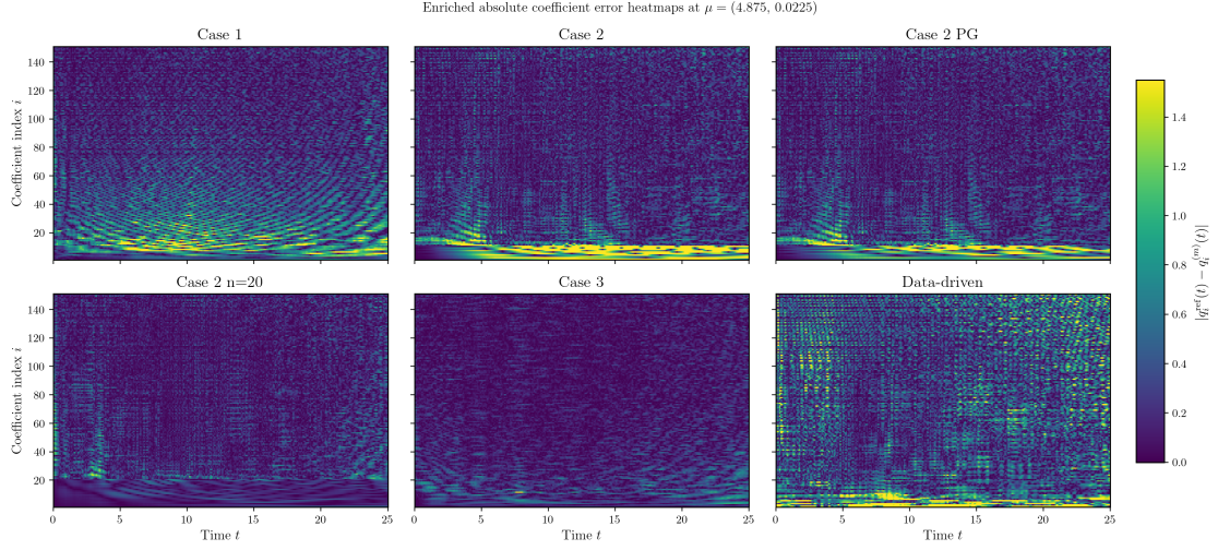
Figure 15: Enriched stage: absolute coefficient error heatmaps at \mu^{(v)} for all available enriched models.
