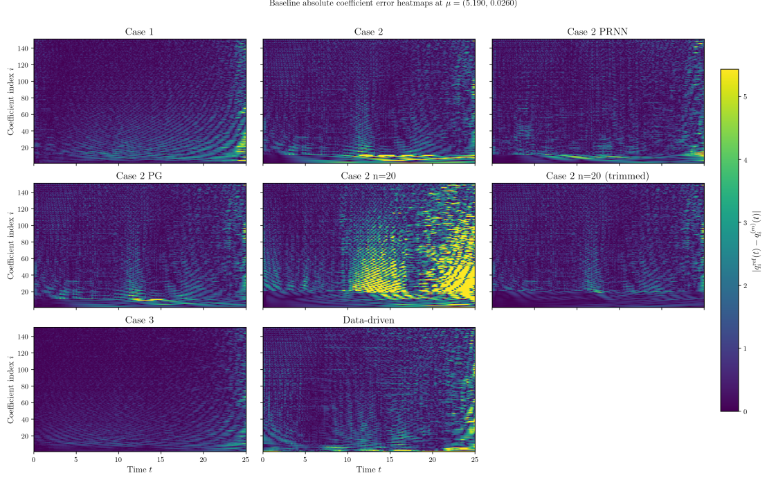
Figure 21: Baseline stage: absolute coefficient error heatmaps at \mu^{(2)} = (5.19, 0.026) for all available baseline models.
