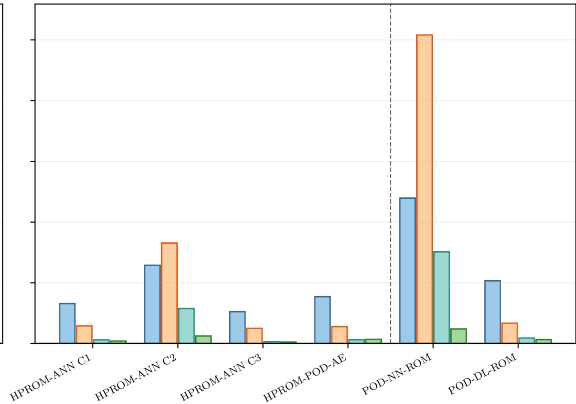
Extrapolation: \mu^{(3)}
