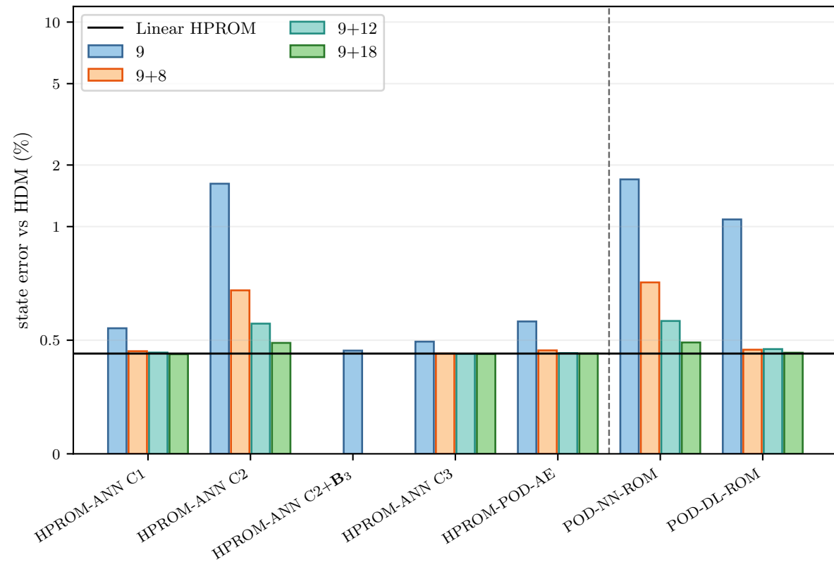
In-domain mean: \mu^{(v)}, \mu^{(1)}, \mu^{(2)}
