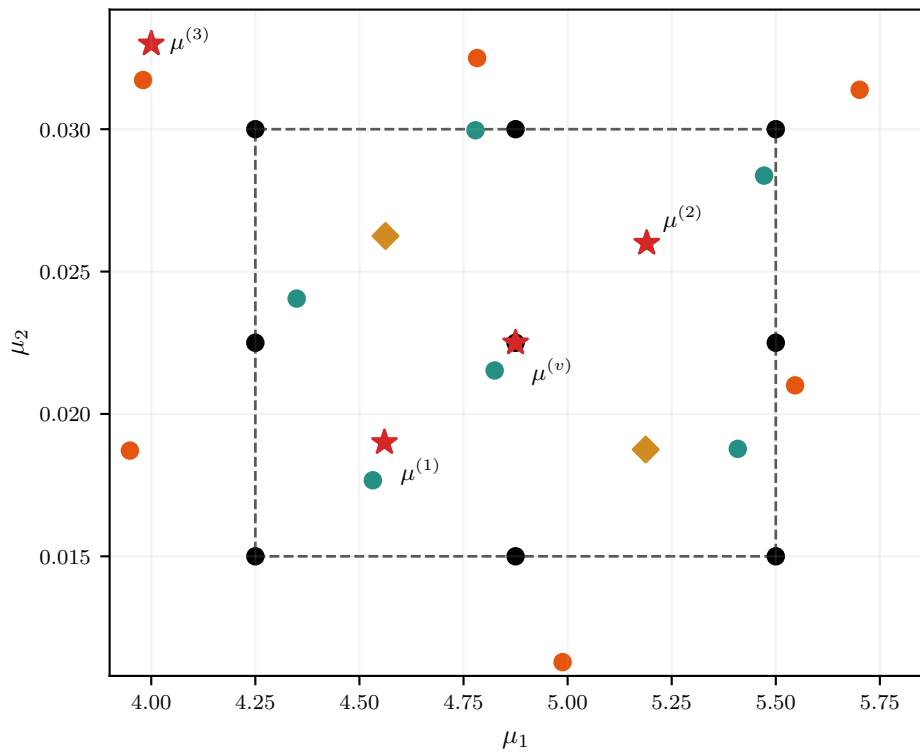
Training trajectories: 9 + 12
