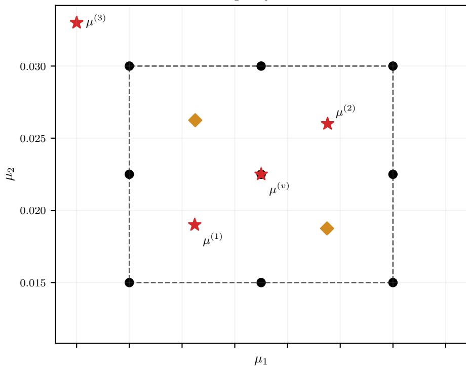
Training trajectories: 9
