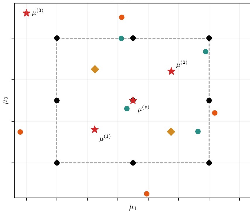
Training trajectories: 9 + 8
