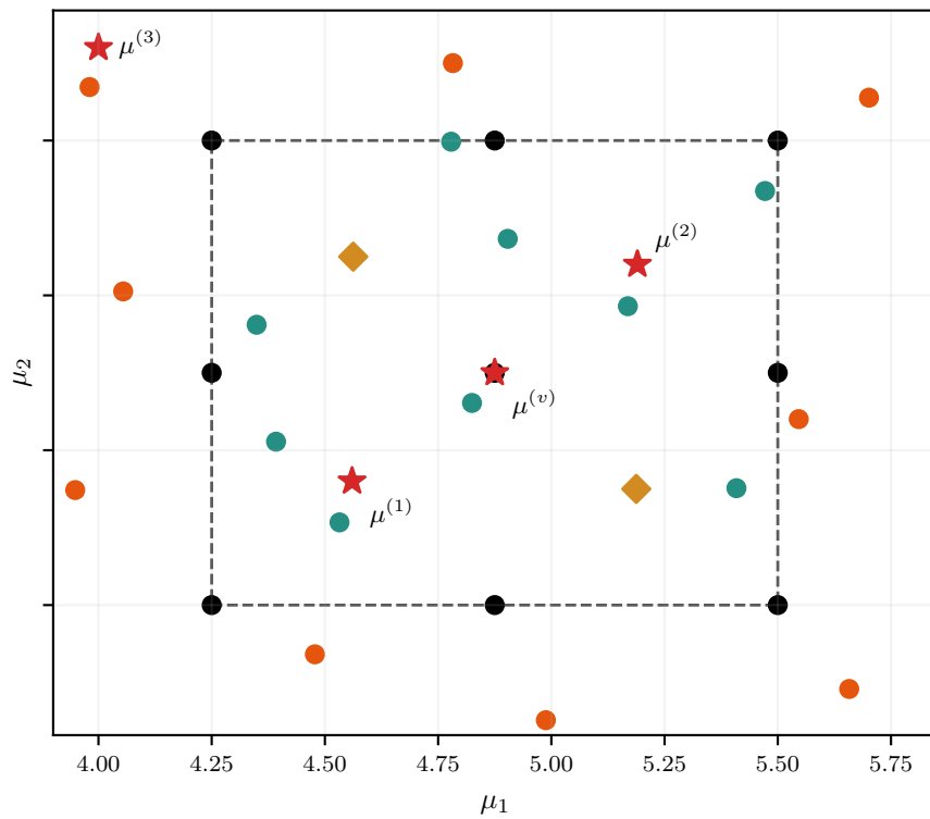
Training trajectories: 9 + 18
