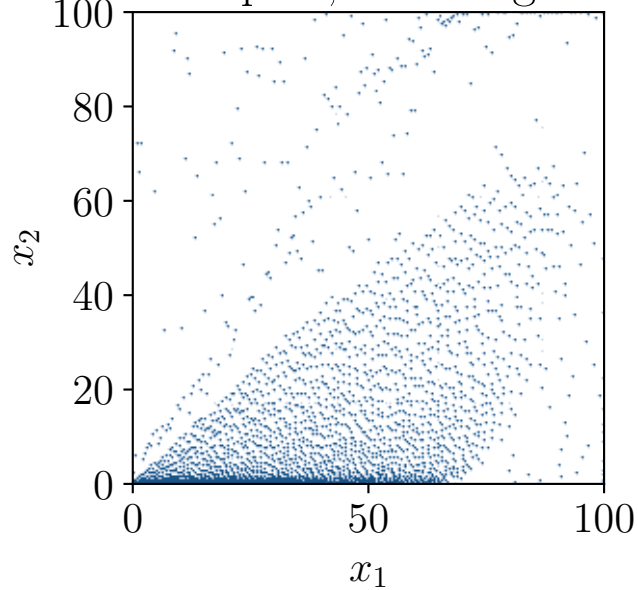
Classical ECSW, offset 1 2492 sampled; 5914 augmented
