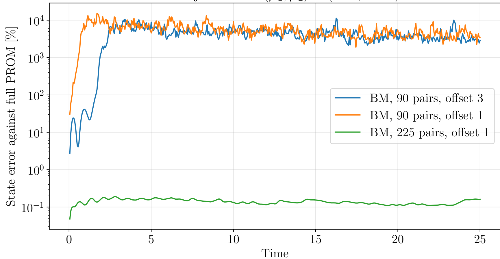
BM trajectories at (\mu_1, \mu_2) = (4.56, 0.019)
