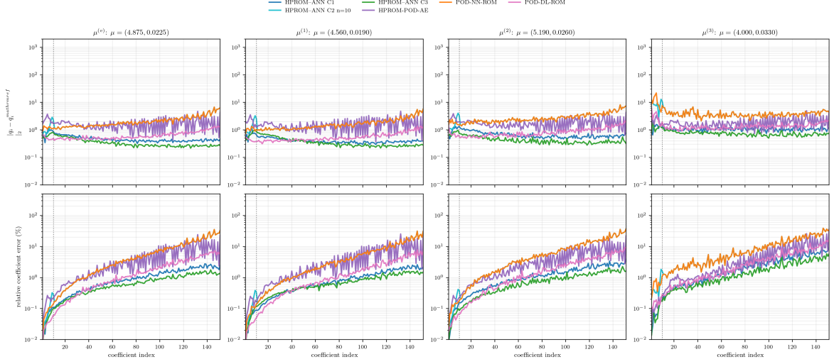
Figure 29: Enriched HPRM online coefficient errors against the enriched linear-HPROM reference. The plotted set is identical to Fig. 20: Case 1, Case 2 with n = 10 , Case 3, PROM-POD-AE, POD-NN-ROM, and POD-DL-ROM. Shared ordinate ranges permit a direct baseline-enriched comparison.
