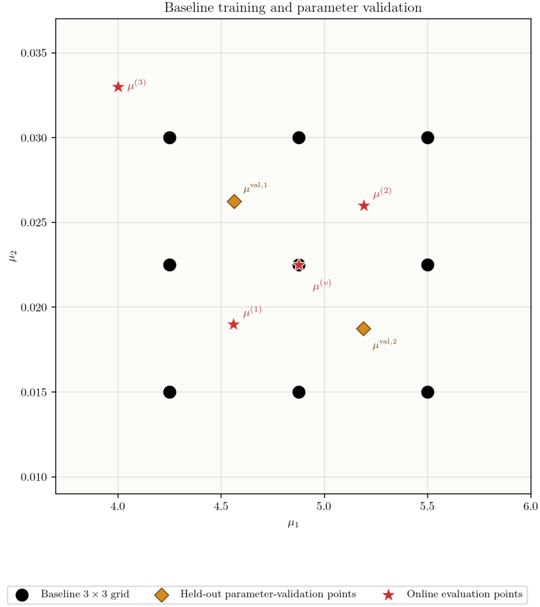
Figure 1: Baseline training, held-out parameter-validation, and online evaluation locations in parameter space. The two diamonds mark \mu^{val,1} and \mu^{val,2} , whose complete linear-PROM or linear-HPROM trajectories are reserved for regression validation. They are distinct from the four red-star online evaluation locations. The axes are shared with the three nested-enrichment designs below.
