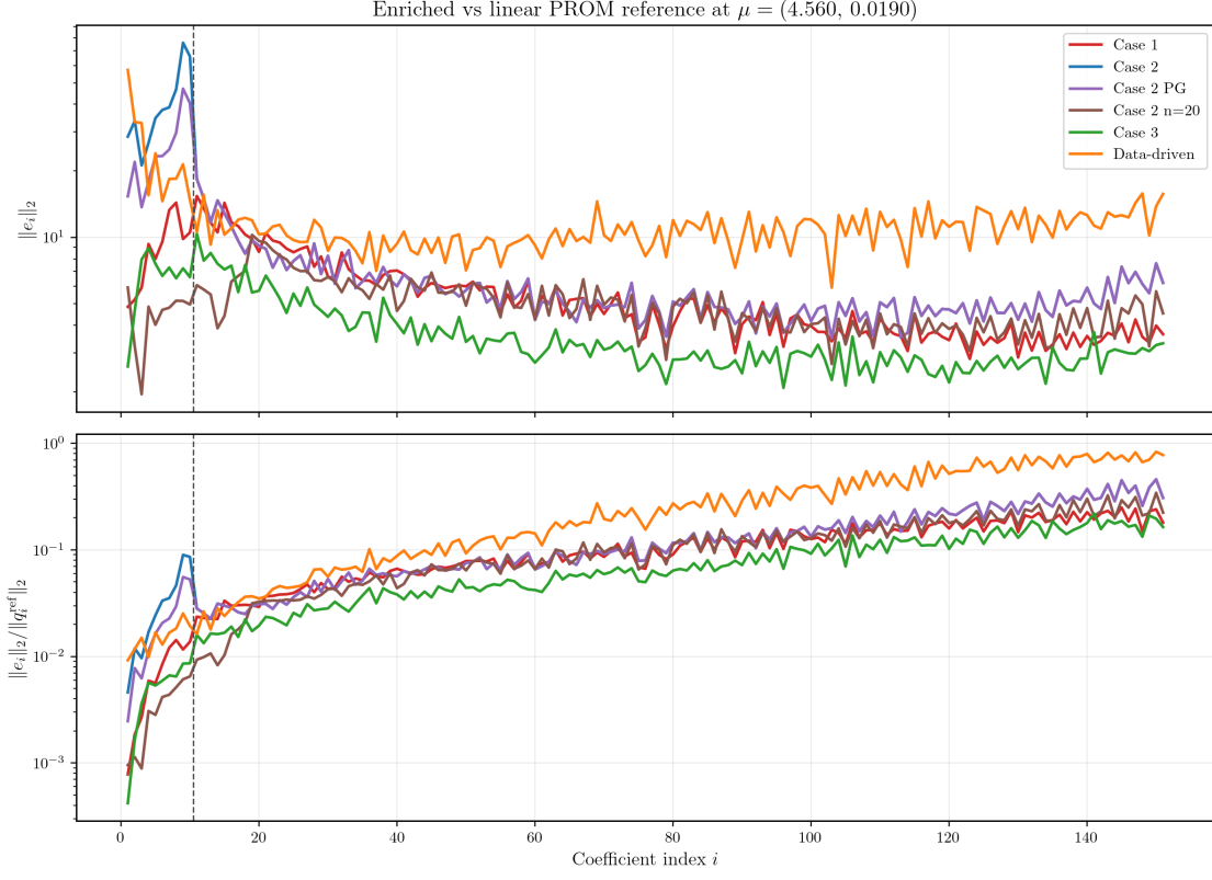
Figure 8: Enriched stage: per-index absolute and relative coefficient errors at \mu^{(1)} = (4.56, 0.019) , including Case 2 PG Oracle and Case 2 n = 20 (native).
