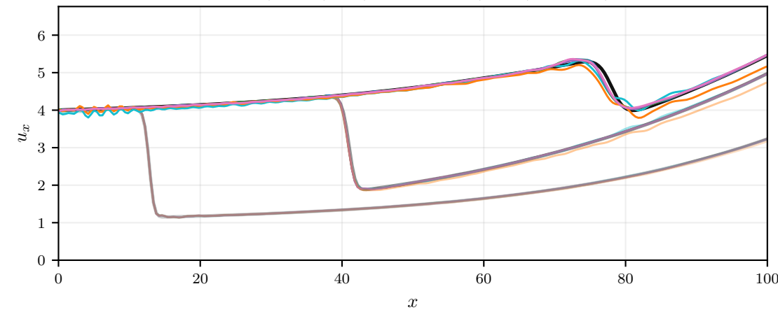
\mu^{(3)}: (\mu_1, \mu_2) = (4.000, 0.0330); u_x(x, y_{mmid})
