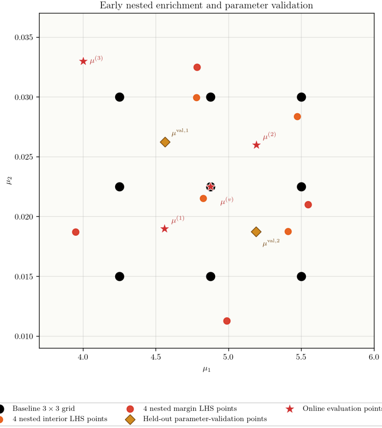
Figure 2: Early nested PROM enrichment. Four interior and four margin points are selected from the fixed full LHS design; they are not a separately sampled design. The four margin representatives cover the left, right, top, and bottom expanded-box directions. The two diamonds and four red stars remain excluded from training. The axes match the other parameter-space figures.
