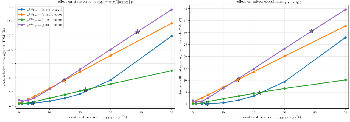
Figure 25: Fixed-rule sensitivity of Case-2 HPROM with n = 10 to secondary-coordinate error. Left: state error against the HDM. Right: error in the ten solved primary coordinates against the linear HPROM. Stars identify the actual master-ANN tail errors.
