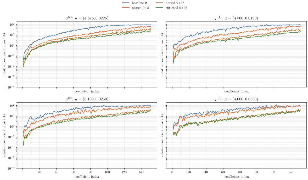
Figure 18: Case-2 per-coefficient relative error across the four-level nested PROM coefficient-data ladder for n = 10 . The vertical line marks the separation between the ten residual-solved primary coordinates and the ANN-injected secondary tail. The linear PROM coefficient trajectory is the reference.
