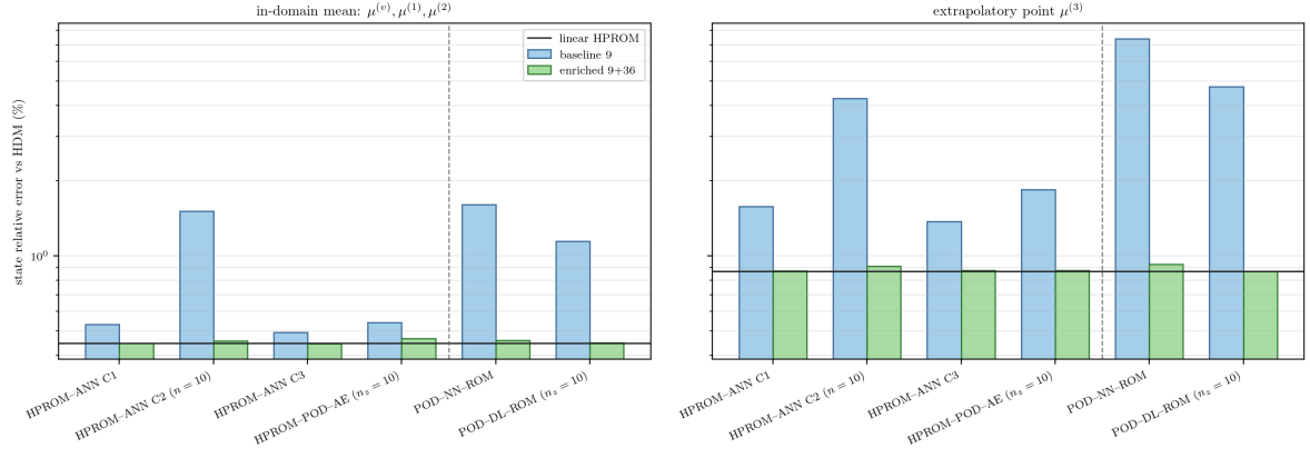
Figure 26: Effect of HPROM coefficient-data enrichment on state error. The black level is the fixed linear HPROM reference; logarithmic axes make both the baseline Case-2 degradation and the enriched recovery visible. The vertical rule separates residual-evaluating intrusive HPROM models from the non-intrusive direct ROM maps.
