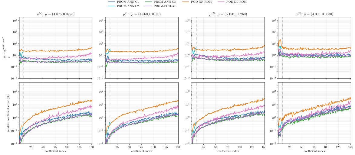
Figure 15: Enriched PROM online coefficient errors against the enriched linear-PROM reference. The plotted set is identical to Fig. 6: Case 1, Case 2 with n = 10 , Case 3, PROM-POD-AE, POD-NN-ROM, and POD-DL-ROM. Shared ordinate ranges permit a direct baseline-enriched comparison.
