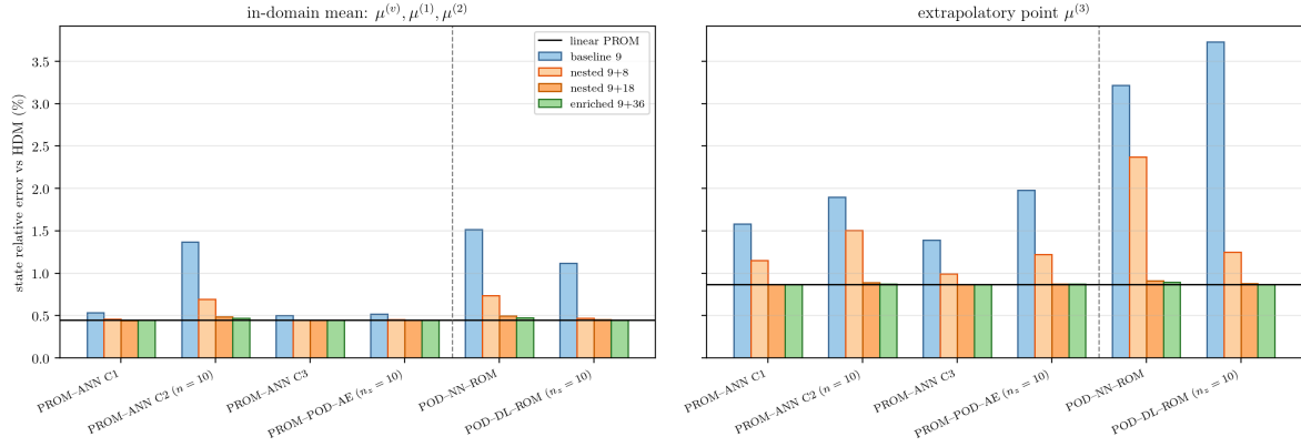
Figure 12: Effect of the four-level nested PROM coefficient-data ladder on online state errors. Left: mean error over the verification and two off-grid in-domain points. Right: extrapolatory point. The vertical rule separates the residual-evaluating intrusive PROM models from the non-intrusive direct ROM maps.
