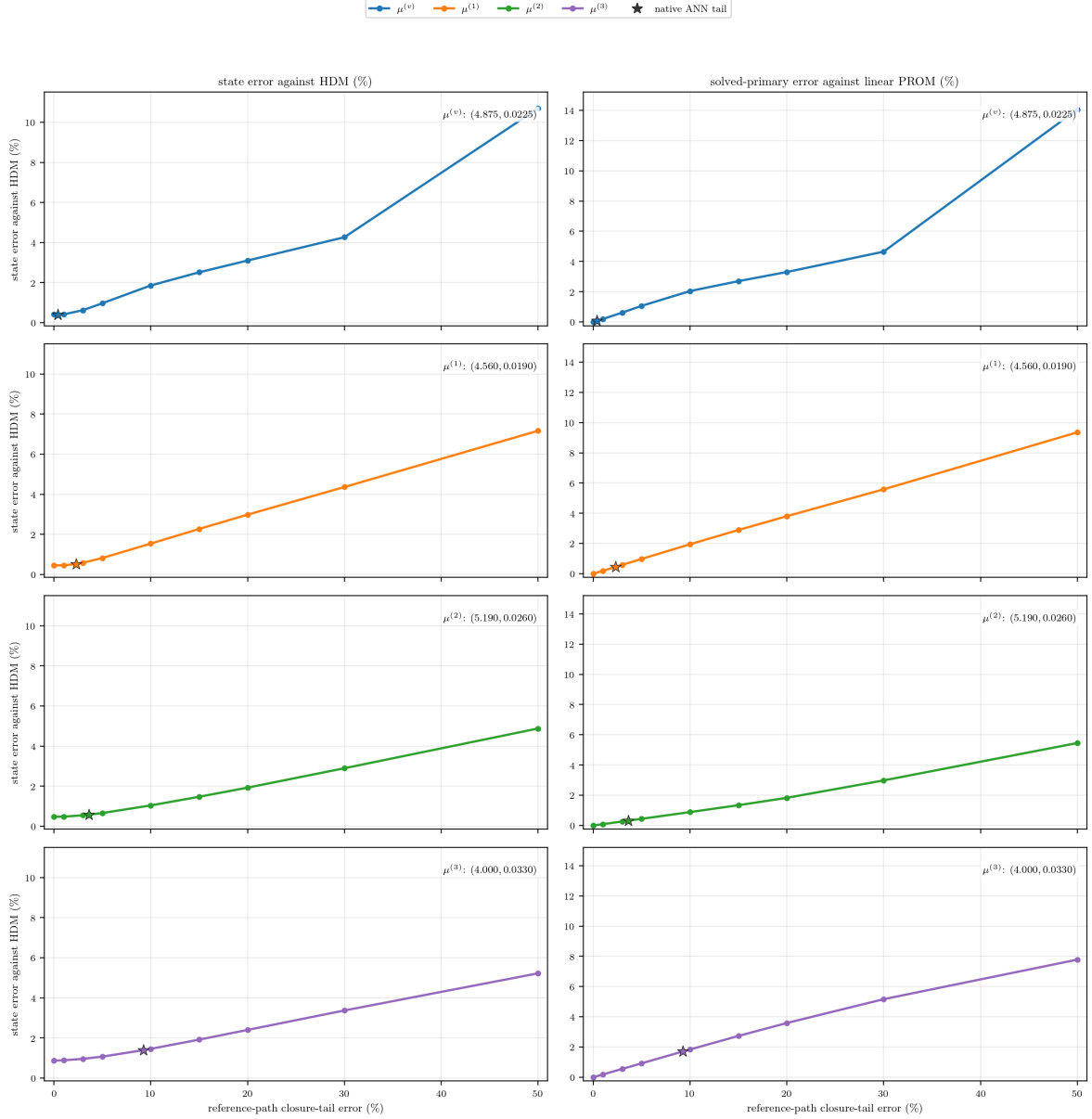
Figure 36: Case-3 tangent-preserving oracle diagnostic, using the same reference-path definition, axes, and star convention as Figure 35. The difference between the prescribed abscissa and the tail error observed along the online trajectory quantifies state-dependent feedback; this is particularly visible at the verification and first off-grid parameters.
