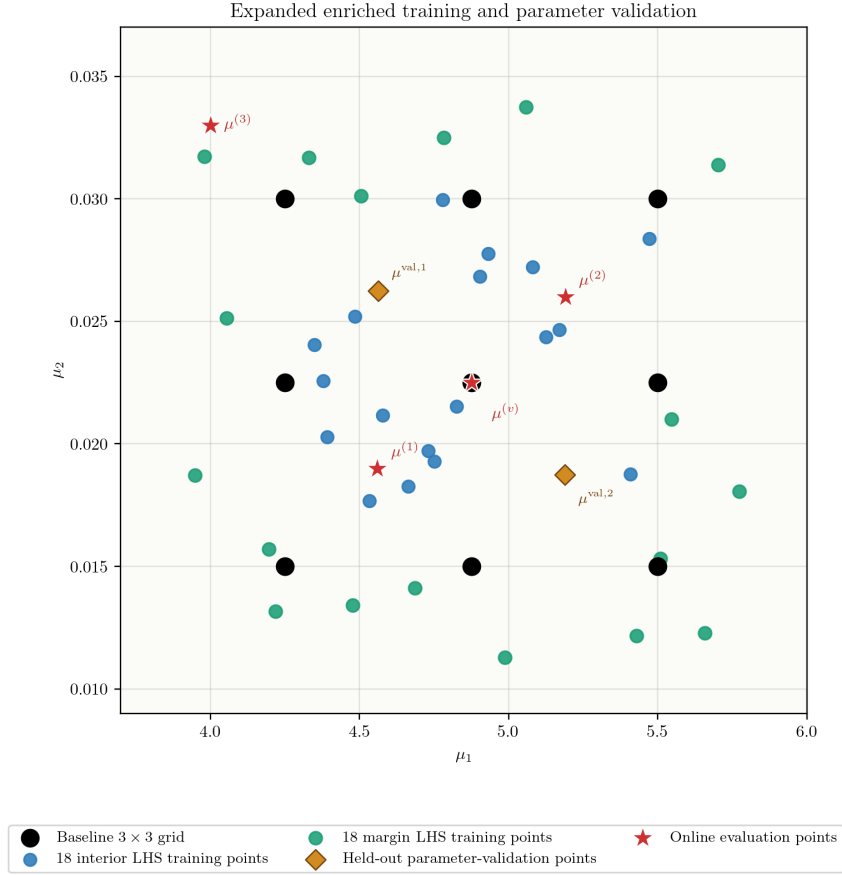
Figure 4: Expanded enriched training, held-out parameter-validation, and online evaluation locations in parameter space. The baseline 3 \times 3 grid is supplemented with the full 18 interior and 18 margin Latin-hypercube training points, generated with the fixed linear teacher in the 25% expanded parameter box. The two diamonds and four red stars are excluded from every training design. The axes match Fig. 1; the enrichment changes coefficient coverage, not the HDM snapshot basis.
