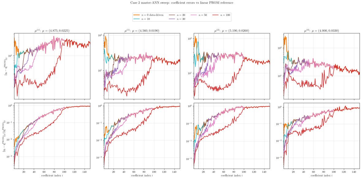
Figure 10: Case-2 PROM coefficient errors with respect to the linear PROM coefficient trajectories for the same n -sweep. Top: absolute time-trajectory error. Bottom: relative error. The dotted vertical line marks coefficient 10, the primary dimension used in the production Case-2 runs.
