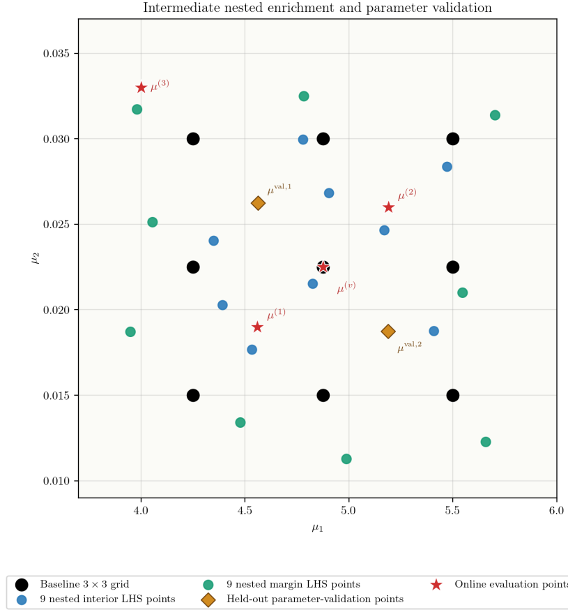
Figure 3: Intermediate nested PROM enrichment. Nine interior and nine margin points are selected from the fixed full LHS design; they are not a separately sampled design. The two diamonds and four red stars remain excluded from training. The axes match Figs. 1, 2, and 4.
