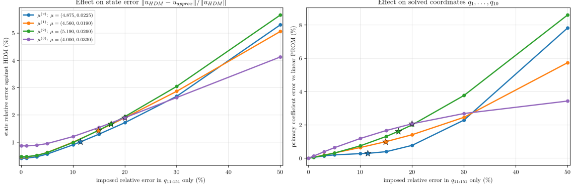
Figure 11: Fixed-split sensitivity of Case-2 PROM with n = 10 to prescribed secondary-coordinate error. Left: state error against the HDM. Right: error in the ten solved primary coordinates against the linear PROM.
