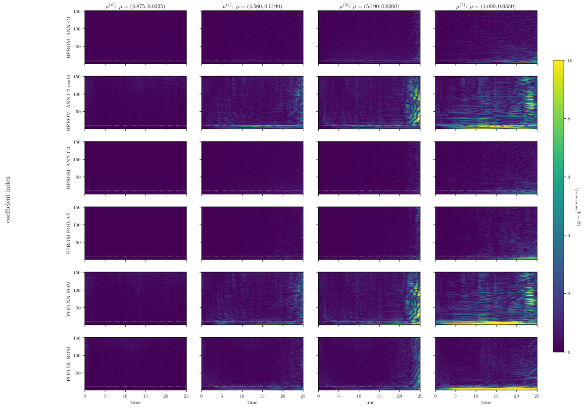
Figure 21: Baseline HPROM time-by-coefficient absolute errors against the linear HPROM. The row/column ordering, the primary-coordinate separator, and the absolute colour range are identical to those of Fig. 7.
