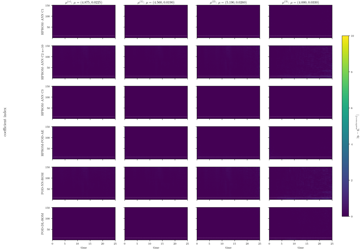
Figure 30: Enriched HPROM time-by-coefficient absolute errors against the enriched linear HPROM. Rows include the four intrusive learned HPROMs followed by POD–NN–ROM and POD–DL–ROM. The colour range and coefficient-10 separator are identical to the baseline HPROM heatmap in Fig. 21.
