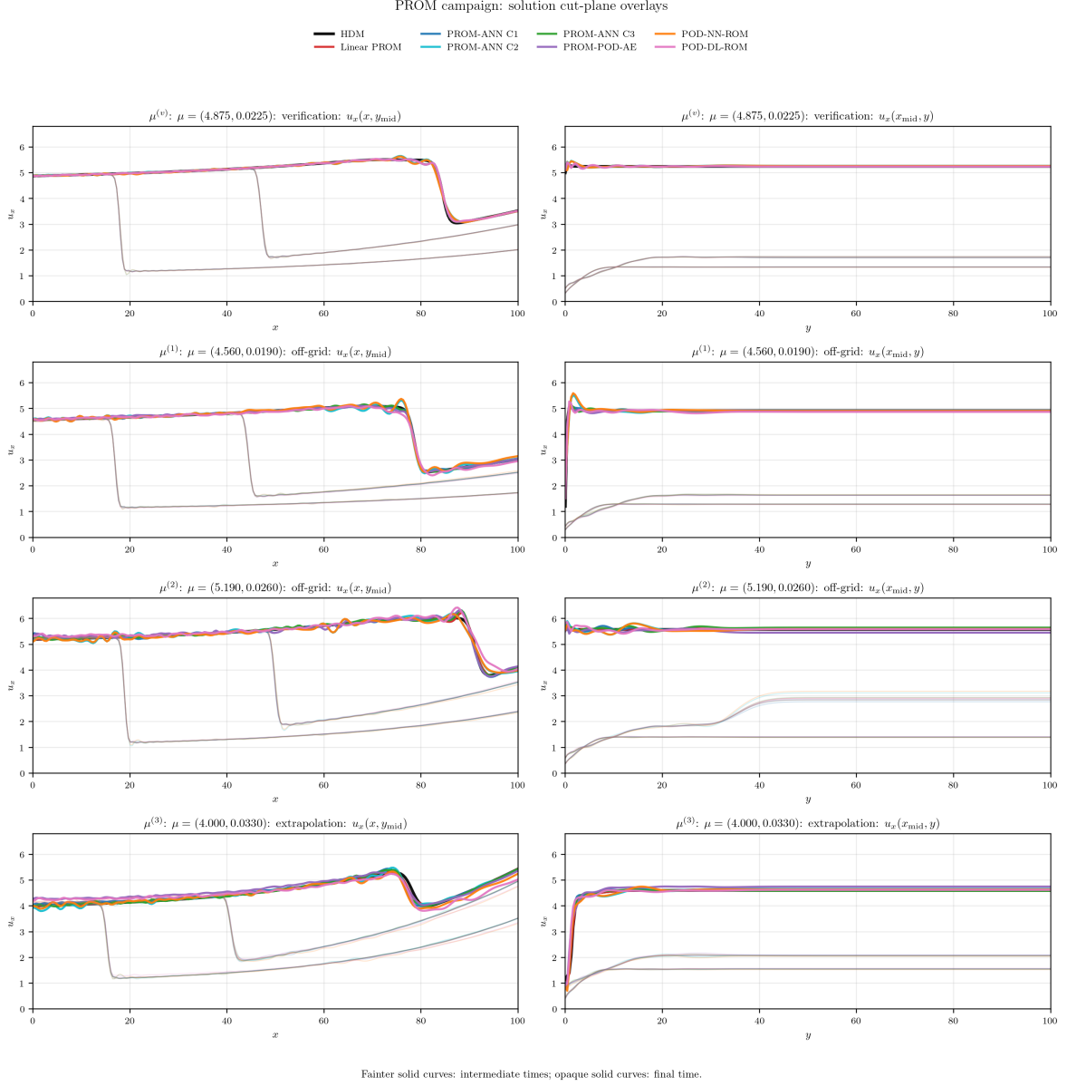
Figure 5: Baseline PROM solution cut-plane comparison against the HDM at the four evaluation points. Each row corresponds to one parameter, with u_x(x, y_{\text{mid}}) at left and u_x(x_{\text{mid}}, y) at right. Fainter solid curves denote the two intermediate times and opaque solid curves the final time. All panels use the same vertical range for u_x , so the visible deviations are directly comparable across parameters and cut planes.
