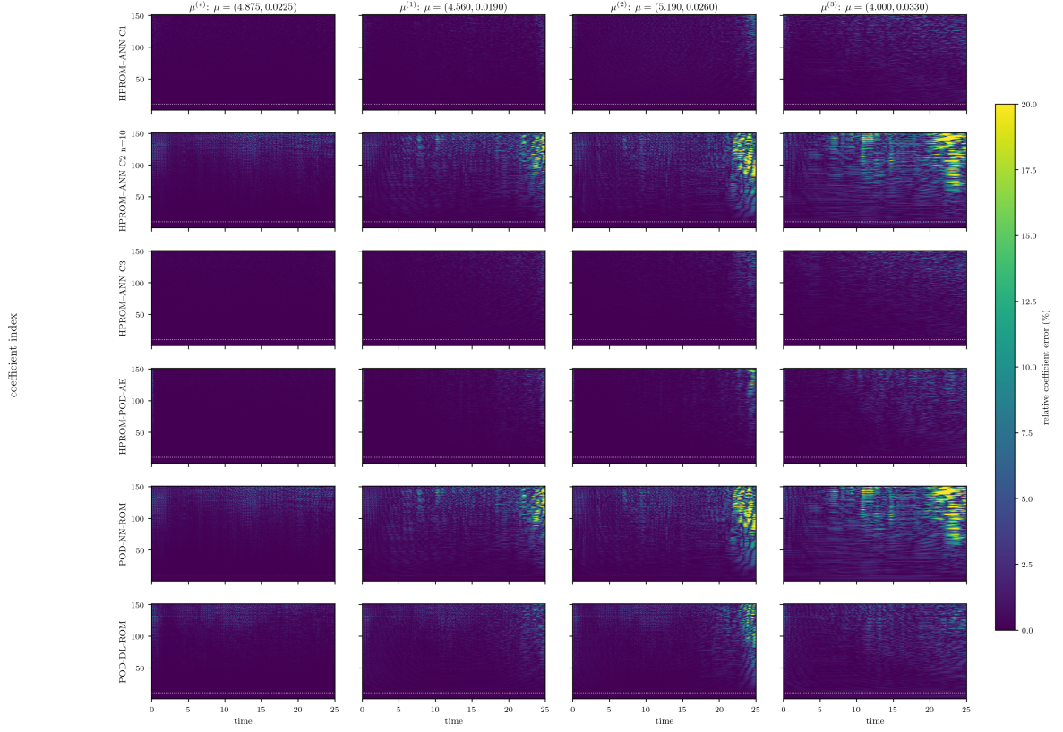
Figure 22: Baseline HPROM time-by-coefficient relative errors against the linear HPROM. The common 0–20% colour range is exactly the one used in Fig. 8; hence colour intensities can be compared directly between the PROM and HPROM panels.
