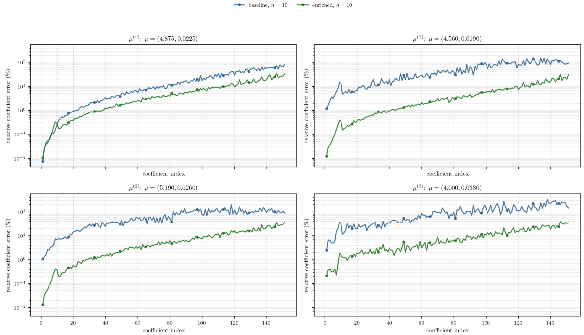
Figure 32: Case-2 per-coefficient HPROM relative error before and after coefficient-data enrichment for n = 10 . The dotted vertical line marks the separation between the ten residual-solved primary coordinates and the ANN-injected secondary tail. The linear HPROM coefficient trajectory is the reference.
