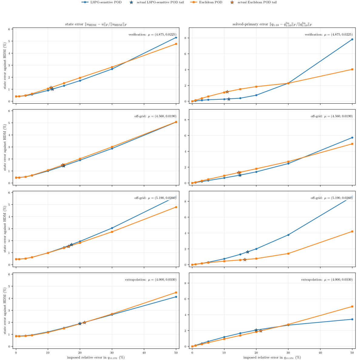
Figure 37: PROM-only controlled secondary-tail comparison for Case-2 with n = 10 . Rows are the verification point, two off-grid points, and the extrapolatory point. Blue circles denote the M -regularized LSPG-sensitive POD basis and orange squares the Euclidean POD basis. Both curves use the same prescribed relative tail-error levels through 50%; stars identify the actual tail-error level of the corresponding master parameter-time map. Left: state error against the HDM. Right: error in the ten solved primary coordinates relative to that basis's own full linear PROM.
