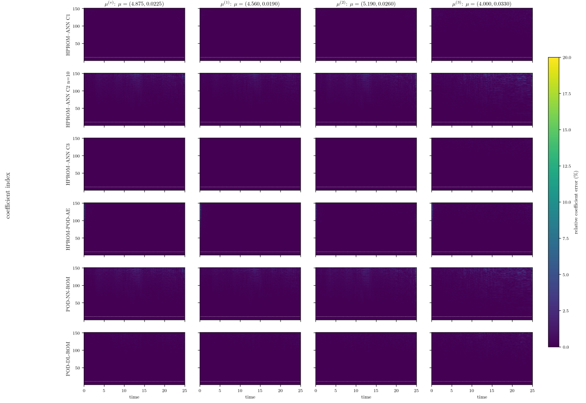
Figure 31: Enriched HPROM time-by-coefficient relative errors. The shared 0–20% colour range exposes the low-error structure recovered by enrichment while clipping only larger values.
