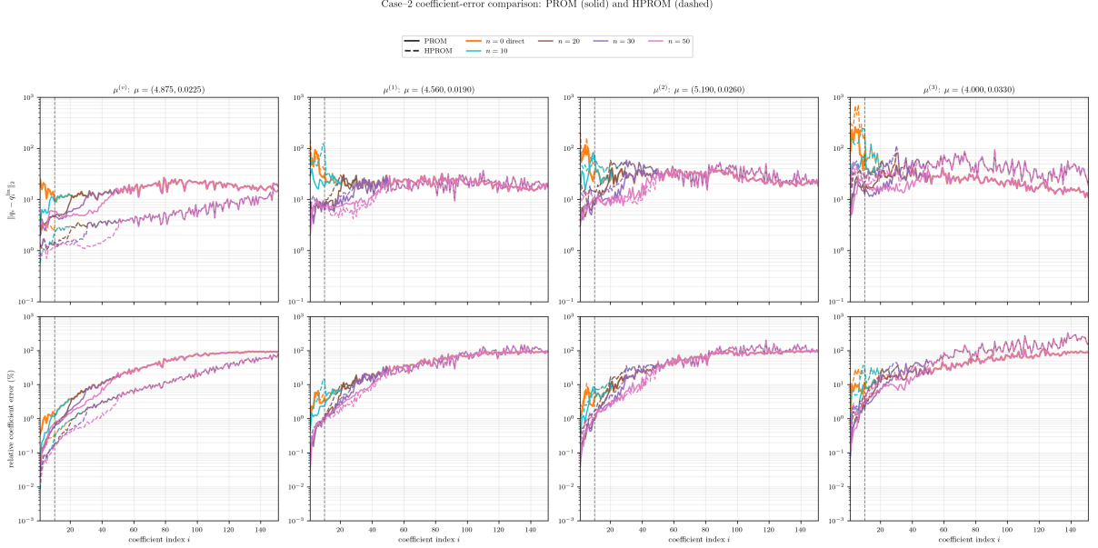
Figure 34: Matched Case-2 coefficient-error sweeps. Columns are ordered as \mu^{(v)} , \mu^{(1)} , \mu^{(2)} , and \mu^{(3)} . Top: absolute time-trajectory coefficient error. Bottom: relative coefficient error. Each colour identifies the solved primary dimension n ; solid curves are PROM and dashed curves are HPROM. The vertical line marks coefficient 10. Each solver is compared with its own full linear reference trajectory, so the figure exposes the effect of hyperreduction on the matched Case-2 coefficient sweep without conflating the two distinct linear references.
