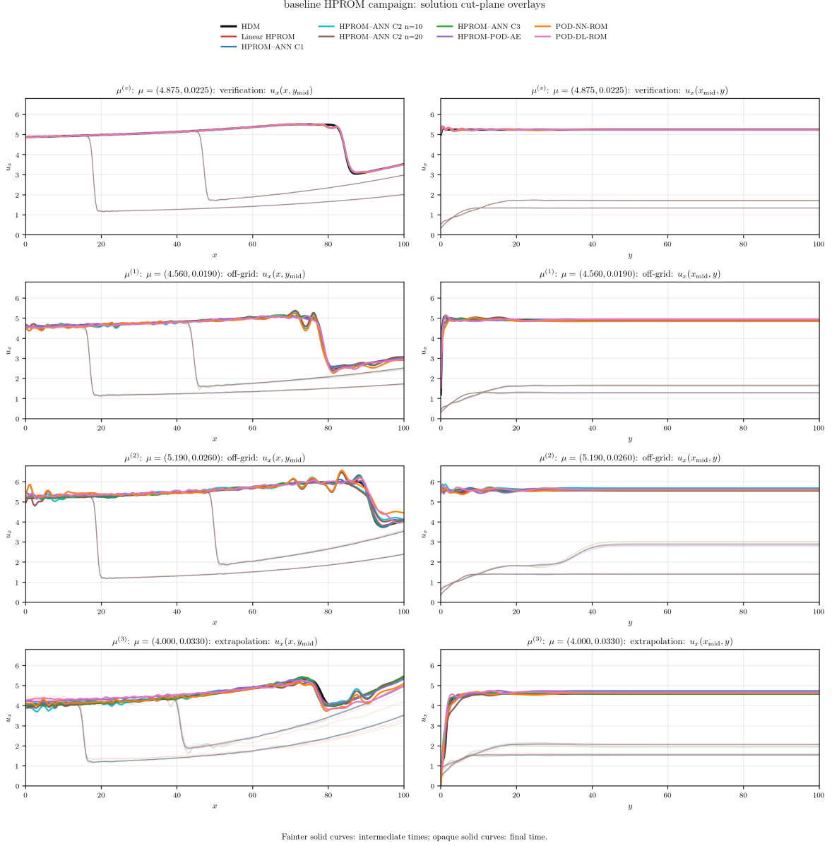
Figure 19: Baseline HPROM solution cut-plane comparison against the HDM at the four evaluation points. The layout, solid-curve time-opacity convention, state range, and method colors are identical to those in Fig. 5. The linear HPROM curves are reconstructed from their saved coefficient trajectories; the nonlinear HPROM curves use the saved online state snapshots.
