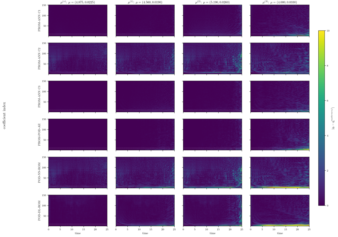
Figure 7: Baseline PROM time-by-coefficient absolute errors |q_i(t) - q_i^{\text{ref}}(t)| against the linear PROM. Columns are ordered as \boldsymbol{\mu}^{(v)} , \boldsymbol{\mu}^{(1)} , \boldsymbol{\mu}^{(2)} , and \boldsymbol{\mu}^{(3)} ; rows identify the online model. The dotted horizontal line is the ten-coordinate primary/secondary split. One common colourbar is used for every panel.
