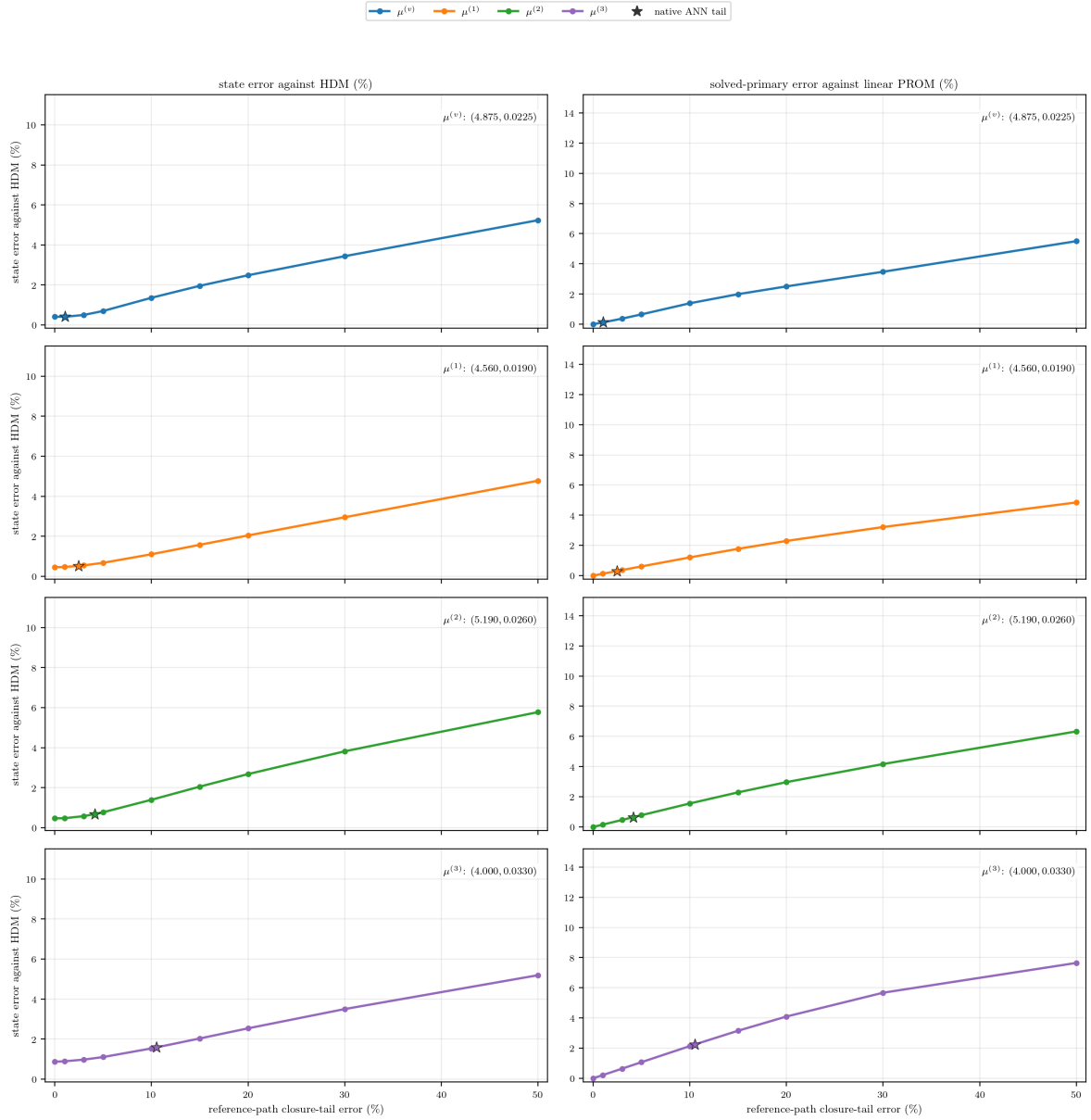
Figure 35: Case-1 tangent-preserving oracle diagnostic. The horizontal axis is the imposed secondary-coordinate discrepancy measured on the linear-PROM reference path. The star marks the native Case-1 ANN tail error, for which the correction in (78) vanishes. Left: state error against the HDM. Right: error in the ten solved primary coordinates against the linear PROM. The ordinate limits are shared with Figure 36.
