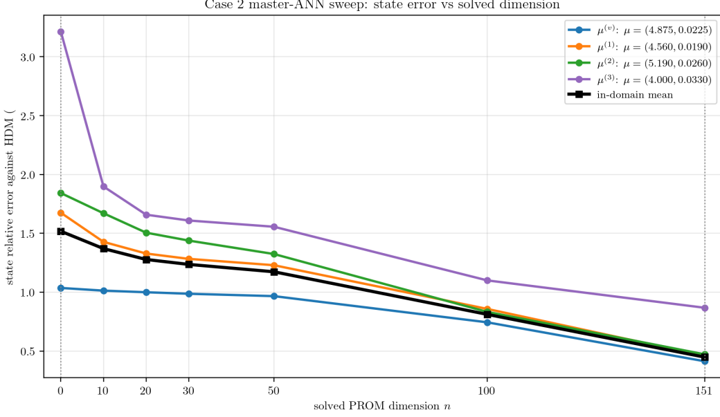
Figure 9: Case-2 PROM state error as the number n of residual-solved primary coordinates is varied. The direct map is the n = 0 endpoint and the 151-coordinate linear PROM is the n = 151 endpoint. The black curve is the in-domain mean over \mu^{(v)}, \mu^{(1)}, \mu^{(2)} ; the extrapolatory point \mu^{(3)} remains a separate curve.
