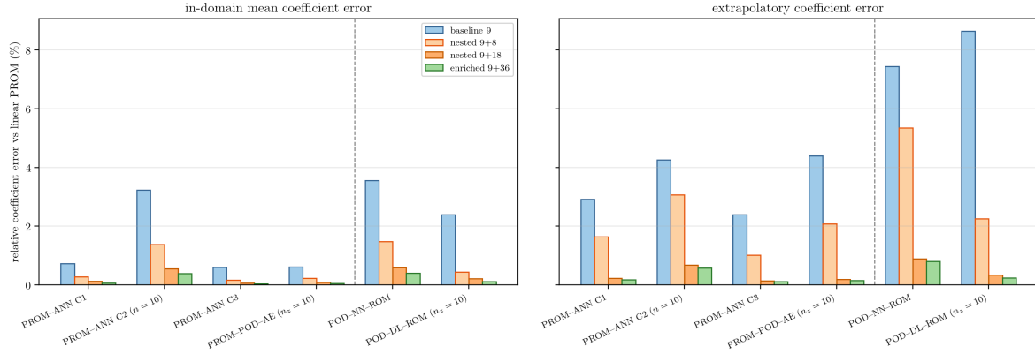
Figure 14: Effect of the four-level nested PROM coefficient-data ladder on online coefficient errors. The coefficient metric is stricter than the state metric because it measures the entire 151-coordinate trajectory against the linear PROM teacher. The vertical rule separates intrusive PROM models from the non-intrusive direct ROM maps.
