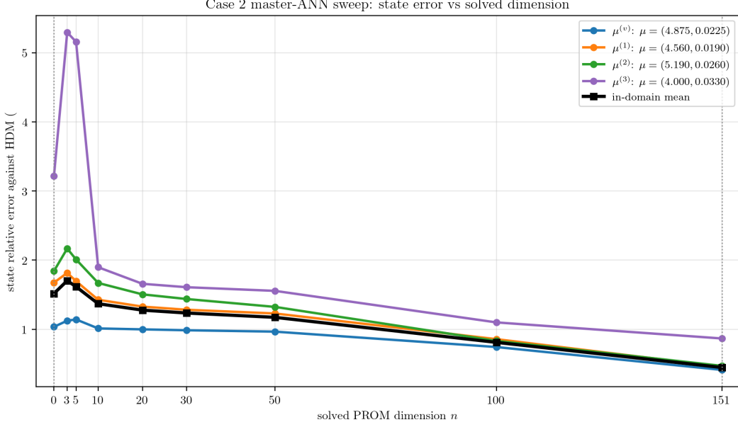
Figure 7: Case-2 PROM state error as the number n of residual-solved primary coordinates is varied. The direct map is the n = 0 endpoint and the 151-coordinate linear PROM is the n = 151 endpoint. The black curve is the in-domain mean over \mu^{(v)}, \mu^{(1)}, \mu^{(2)} ; the extrapolatory point \mu^{(3)} remains a separate curve.
