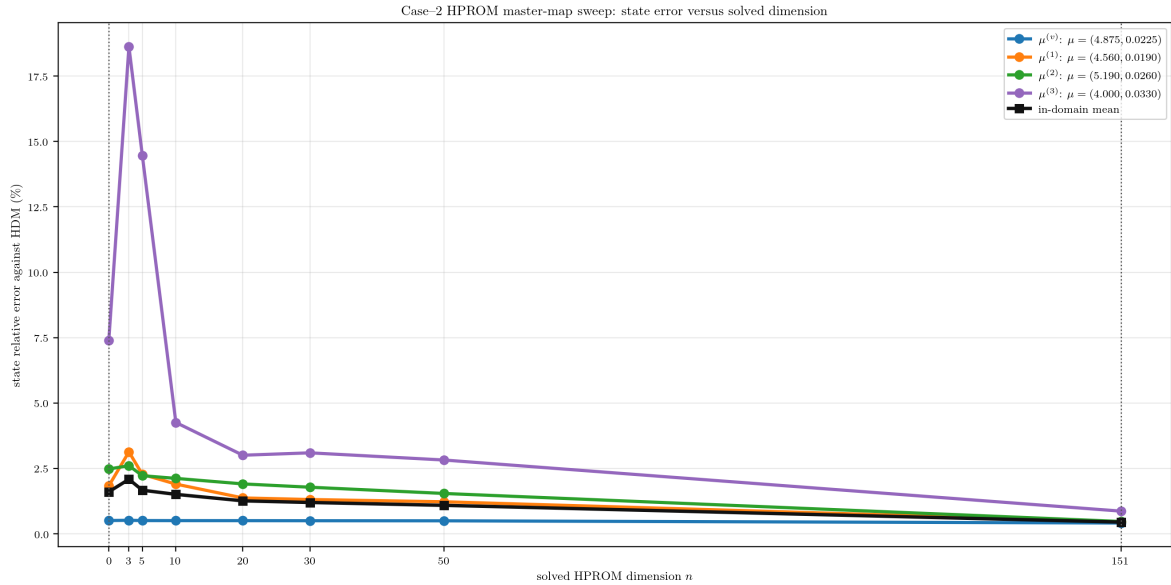
Figure 21: Case-2 HPROM state error as the number n of residual-solved primary coordinates is varied. Each intermediate point uses its matched 2% ECM rule. The dotted horizontal levels are the 151-coordinate linear-HPROM errors.
