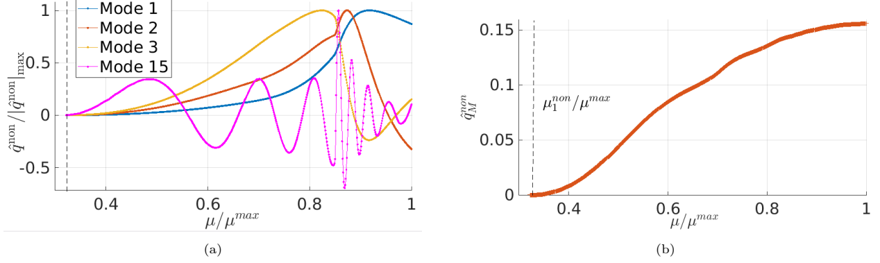
Figure 15: Identification of the nonlinear latent coordinate for the damage benchmark. The horizontal axis represents the normalized load parameter \mu/\mu^{\text{max}} for the nonlinear portion of the training tensile test (see expression 101). (a) Components 1, 2, 3, and 15 of the normalized nonlinear coordinate vector \hat{\mathbf{q}}_M^{\text{non}} \in \mathbb{R}^{n_\Phi-1} , where n_\Phi = 16 ; see Eq. 100. (b) Normalized latent variable \hat{q}_M^{\text{non}} obtained as a linear combination of \hat{\mathbf{q}}_M^{\text{non}} ( \hat{q}_M^{\text{non}} = \mathbf{H}_M^{\text{non}} \hat{\mathbf{q}}_M^{\text{non}} ). The matrix of coefficients in this linear combination, \mathbf{H}_M^{\text{non}} , is determined by solving the generalized eigenvalue problem (102).
