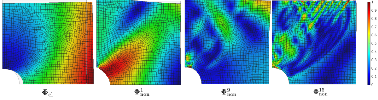
Figure 12: Elastic mode \Phi^{\text{lin}} \in \mathbb{R}^N and three representative nonlinear modes from \Phi^{\text{non}} \in \mathbb{R}^{N \times n_\Phi - 1} ( N = 19832 , n_\Phi = 16 ), obtained from the displacement snapshots generated along the monotonic training trajectory shown in Figure 11(b). The deformed configurations are displayed together with contour plots of the Euclidean norm, normalized by its maximum value.
