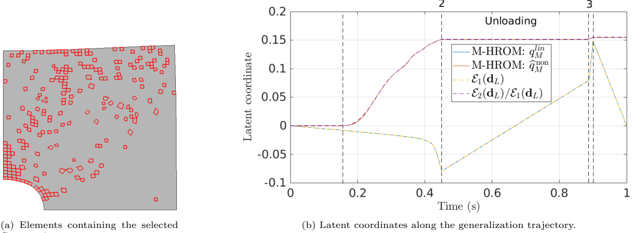
Figure 17: Fixed-weight manifold HROM for the damage benchmark. (a) Elements containing the 277 Gauss points selected by the ECM. (b) Evolution of q_M^{lin} and \hat{q}_M^{non} along the generalization trajectory of Fig. 11(c), compared with the coordinates obtained by applying the encoder in Eq. 29 to the FE solutions.
