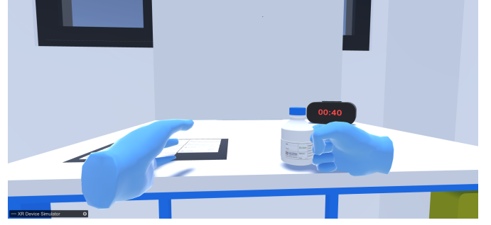
Fig. 1. Operator view of the immersive labeling workstation. The virtual hands, bottle, label, timer, and spatial work area form the human-facing layer of the system.
