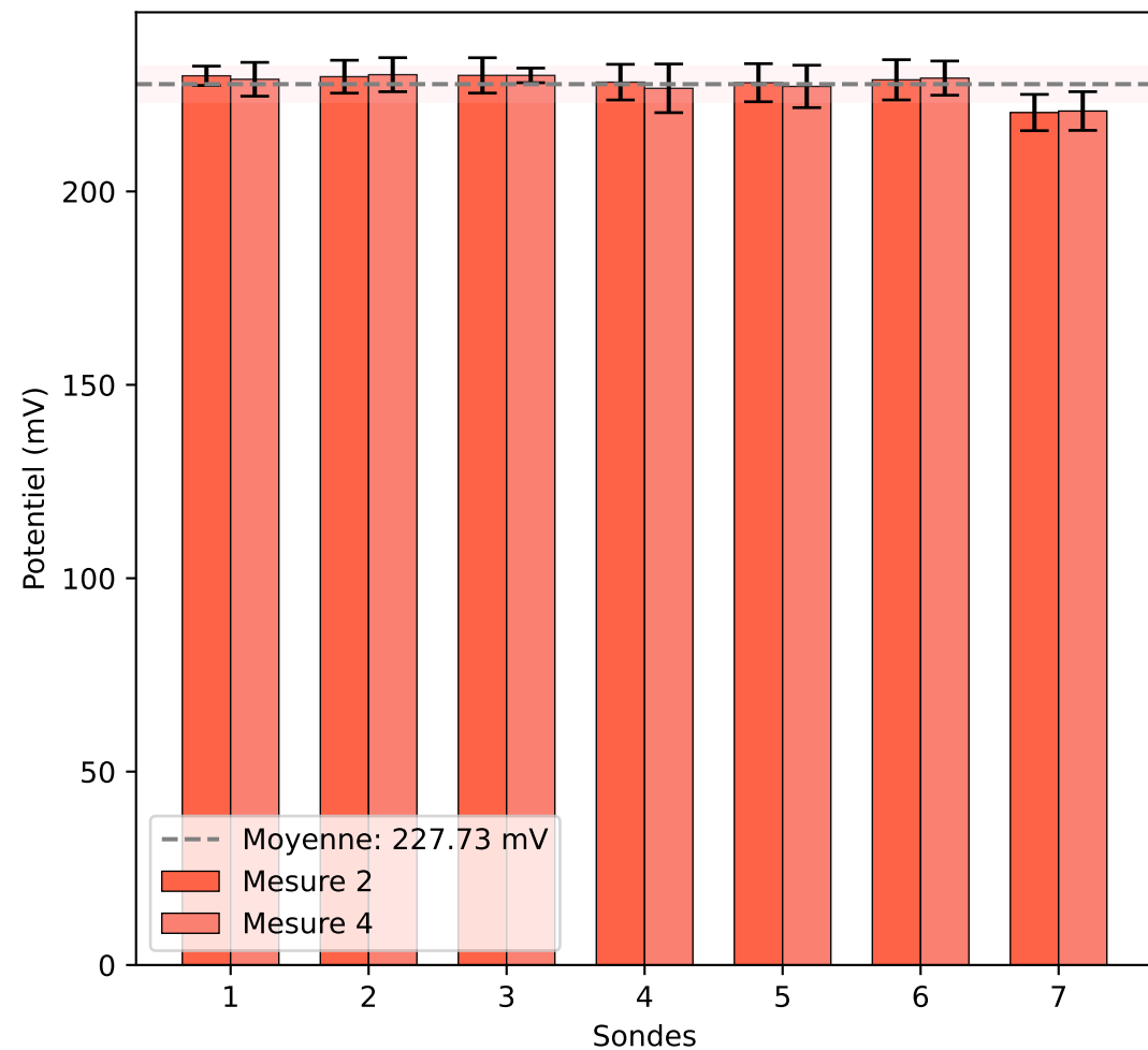
Solution calibrée (240 mV)
