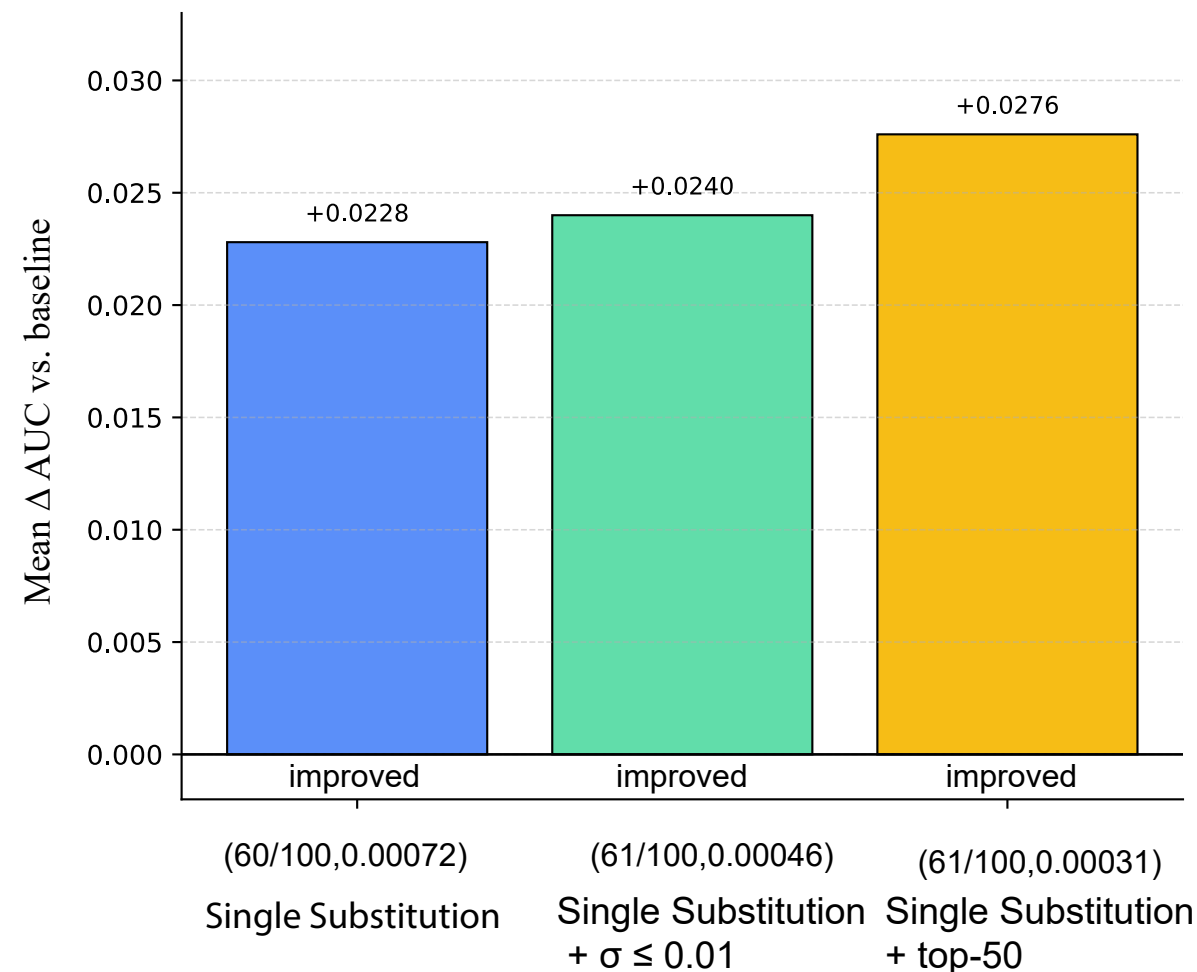
B. ProteinGym Similarity100 Benchmark
