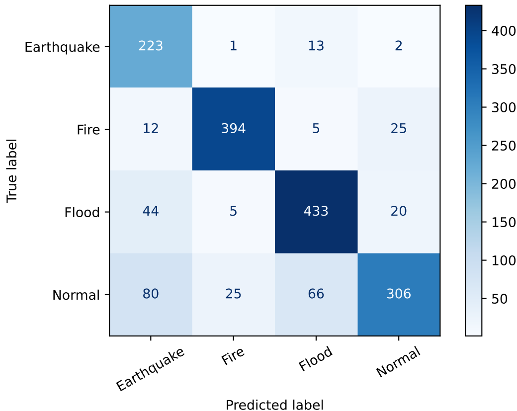
Confusion Matrix — Custom CNN
