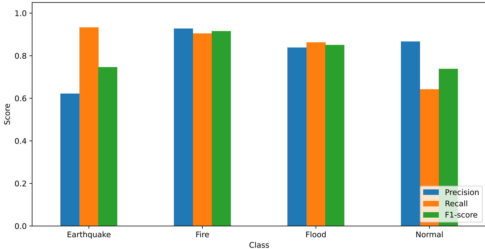
Per-Class Metrics — Custom CNN
