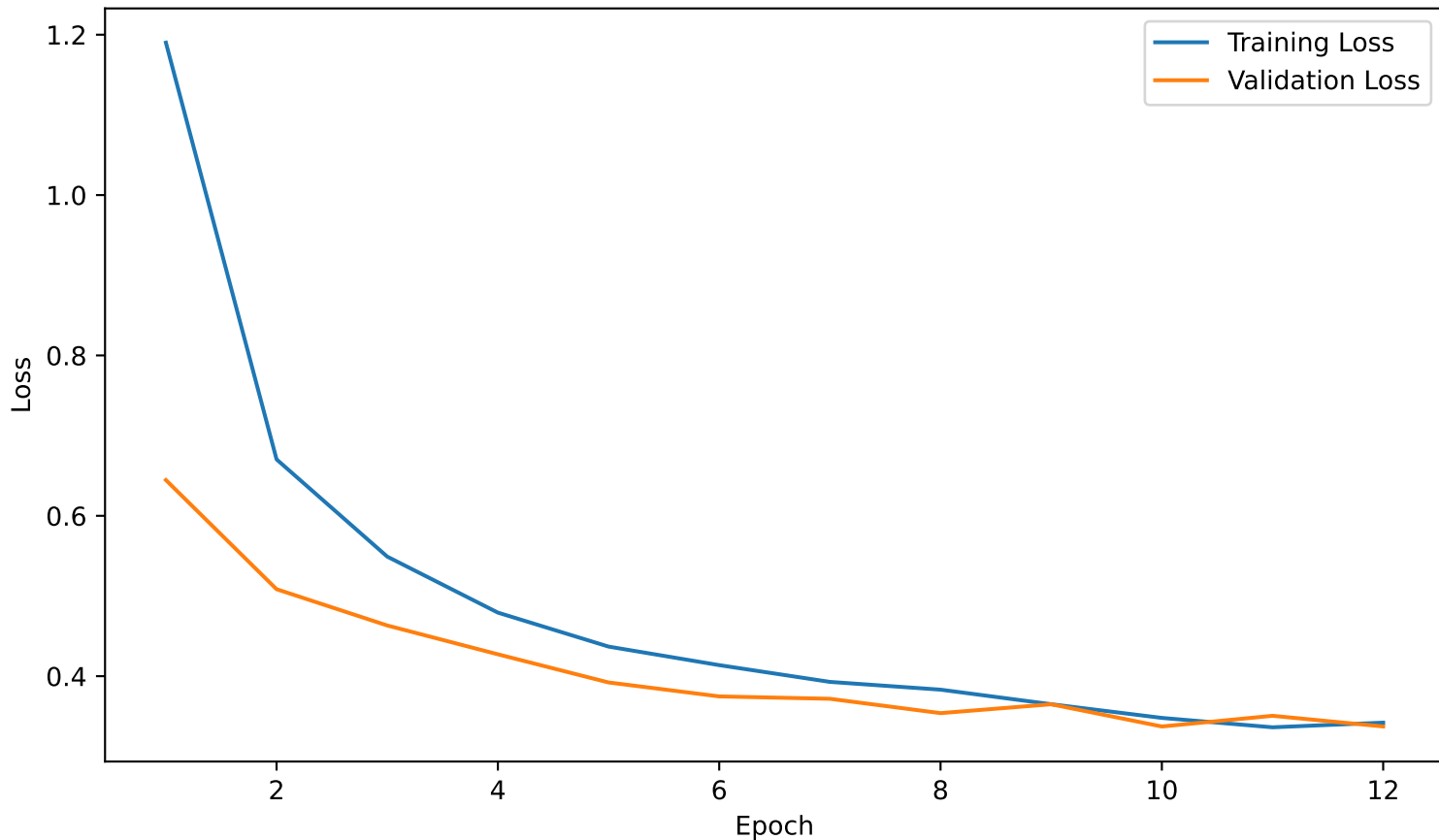
MobileNetV2 Transfer Learning — Loss
