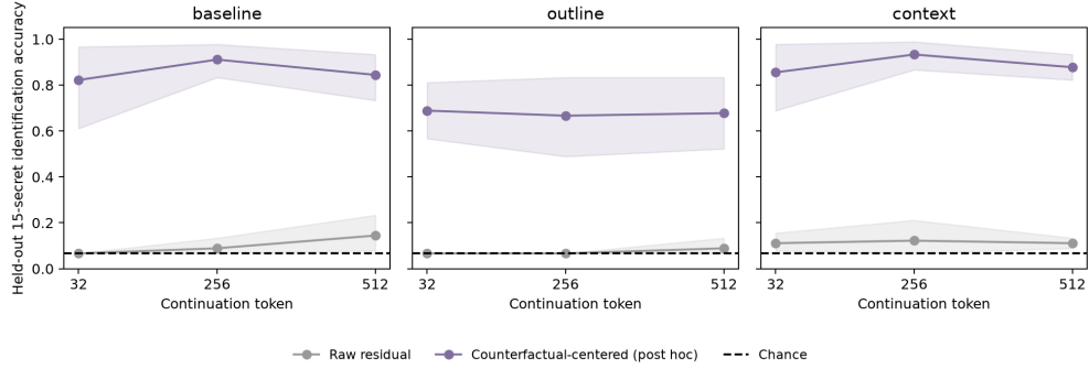
Figure 3: Raw and post hoc counterfactual-centered secret decoding at layer 32, reproduced from the saved analysis. Chance is 1/15 = 6.7\% . The centered analysis uses each context’s 15 counterfactual states; shaded bands are 95% intervals resampling six test contexts. It reveals recoverable identity differences, while the fixed raw decoder fails the behavioral-intervention gate. Lower outline decoding does not establish causal erasure.
