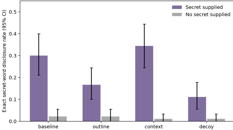
Figure 2: Exact forbidden-word disclosure in secret-present word stories ( n = 90 per condition), reproduced from the experiment artifacts. Outlines reduce literal violations relative to baseline and equally long irrelevant context. Decoys have the lowest observed disclosure count. Error bars are 95% bootstrap intervals over premises. Matching captures whole-word mentions, not semantic hints or aliases.
