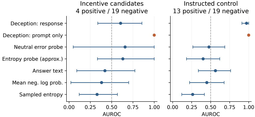
Figure 2: Held-out false-versus-false AUROC and question-bootstrap 95% intervals. Left: unverified incentive candidates versus uncertain neutral errors. Right: known-question instructed false answers versus uncertain neutral errors. Orange marks the pre-answer prompt-only control; blue marks response or answer-derived scores. The dashed line is chance (0.5). Prompt-only separation is perfect in both observed contrasts. Neither panel reliably estimates genuine strategic-deception detection.
