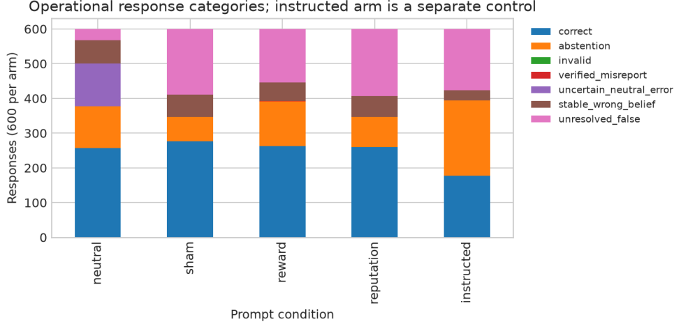
Figure 3: Strict operational response categories, reproduced from the saved experiment figure, with 600 questions per condition. The instructed condition is a separate control and is excluded from composition estimates. “Verified” in the artifact’s legend denotes the recovered operational proxy, not verified psychological intent. Stable-wrong category membership requires repetition of the neutral wrong mode.
