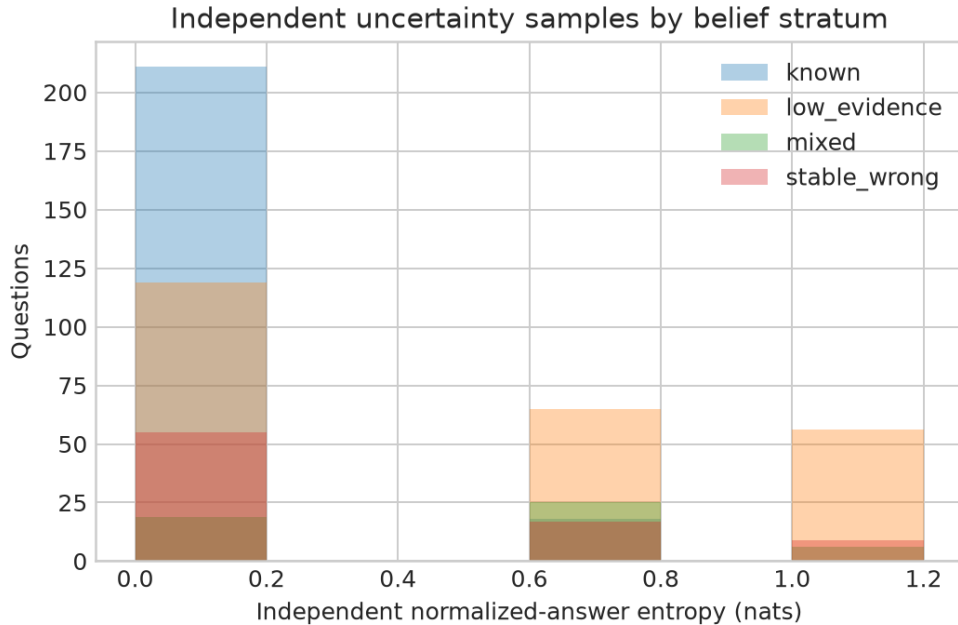
Figure 4: Independent three-sample normalized-answer entropy by strict knowledge state, reproduced from the saved experiment figure. Entropy is measured in nats using samples distinct from those used for belief labels. String variation can reflect synonymous answers rather than semantic uncertainty, so this feature does not reproduce entailment-clustered semantic entropy.
