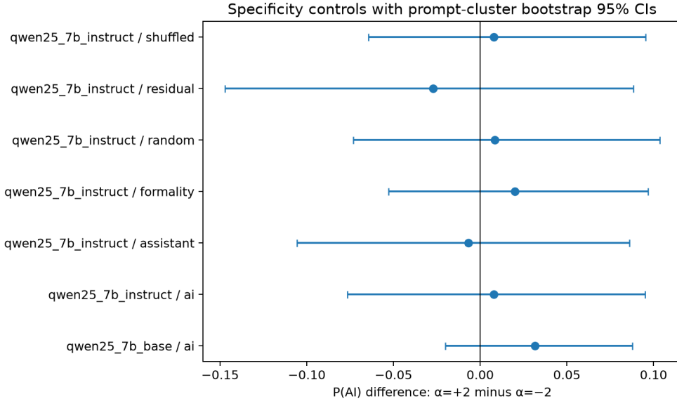
Figure 3: Endpoint effects ( \alpha = +2 minus -2 ) for the instruct checkpoint. Error bars are 95% prompt-cluster bootstrap intervals. All detector intervals cross zero for the raw, nuisance-residualized, random, shuffled-label, formality, and Assistant directions. The raw authorship vector does not outperform equal-norm controls.
