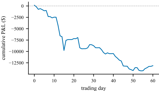
Paper equity across all strategies
